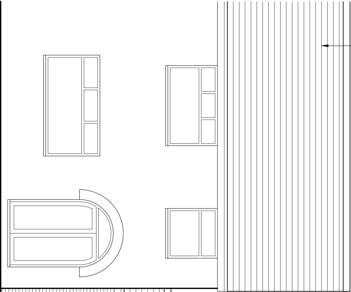
Proposed Front Elevation 1:50
