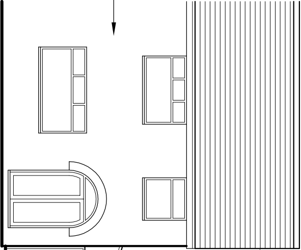
Existing Front Elevation 1:100
