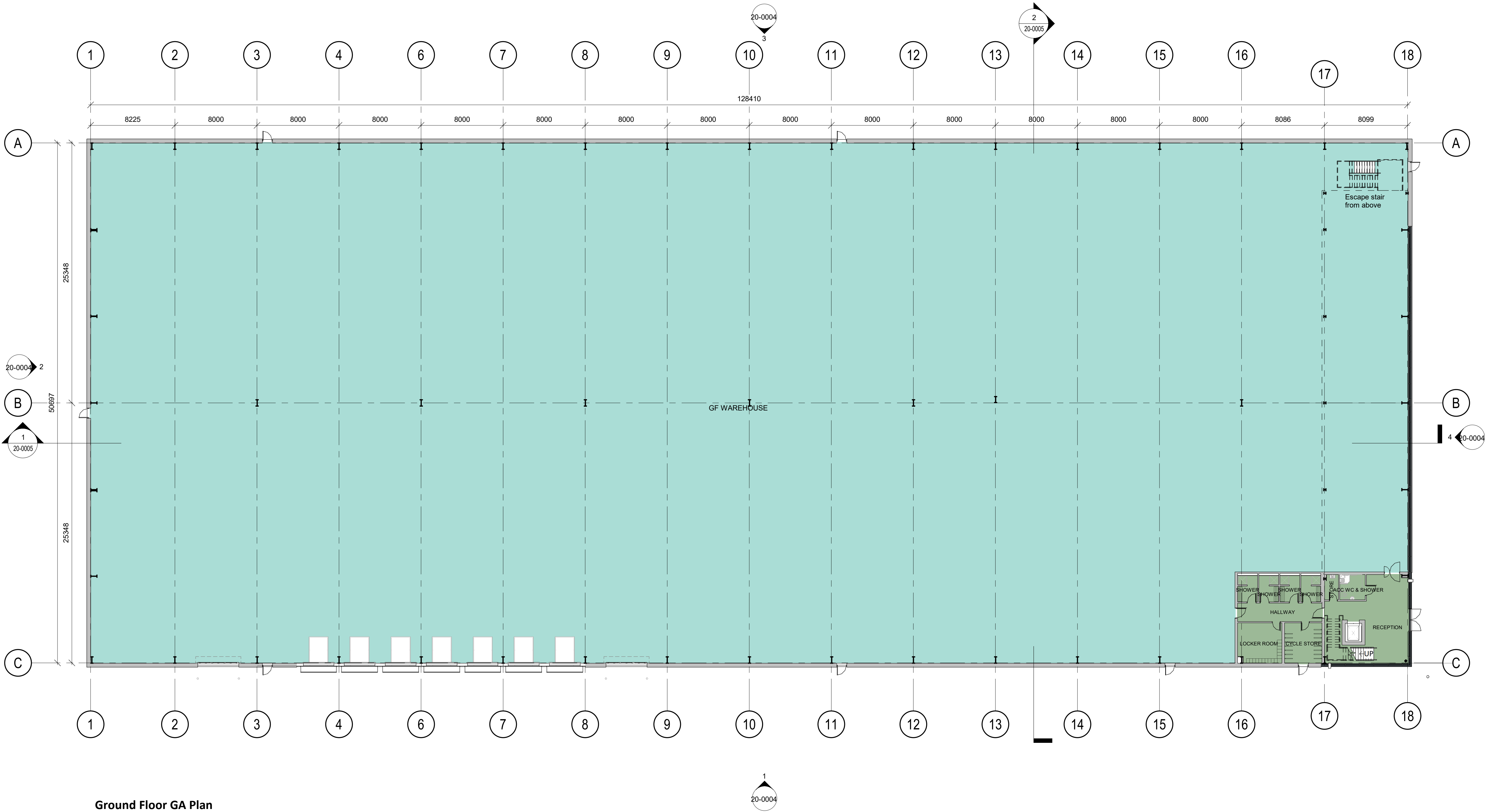
Ground Floor GA Plan 1 : 200
