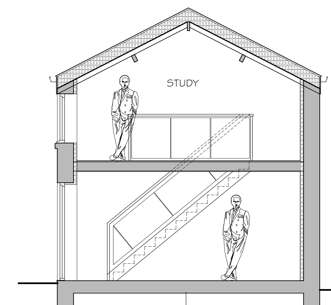
PROPOSED SECTION G-G (1:50)
