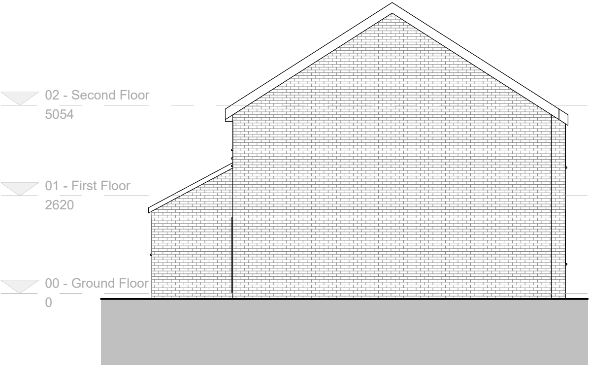
Left Side Elevation - Proposed
