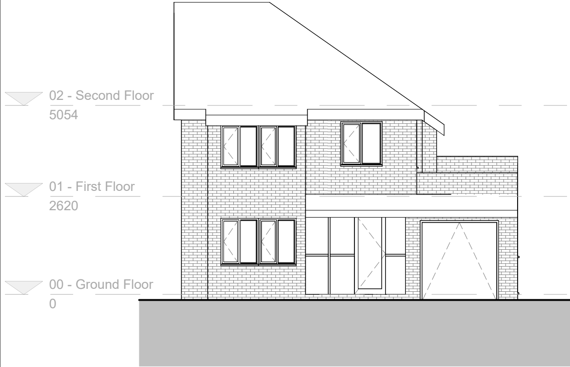
Front Elevation - Existing
