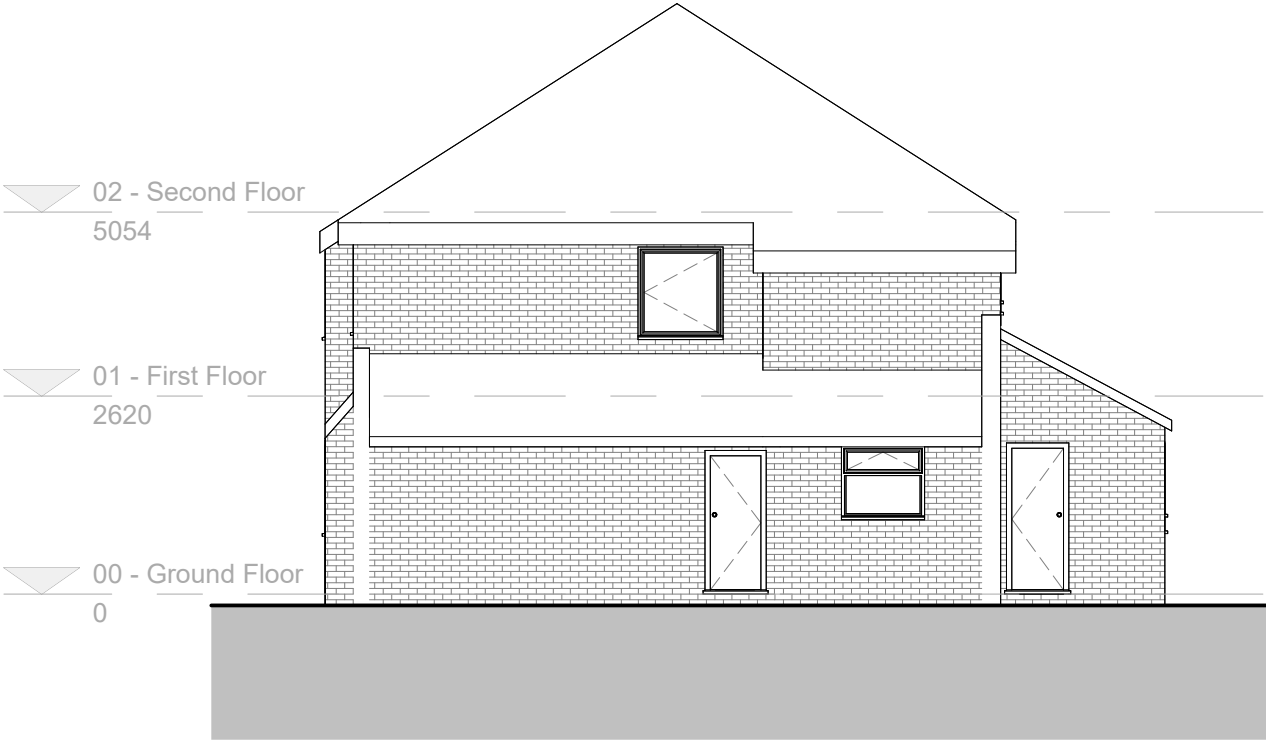
Right Side Elevation - Existing
