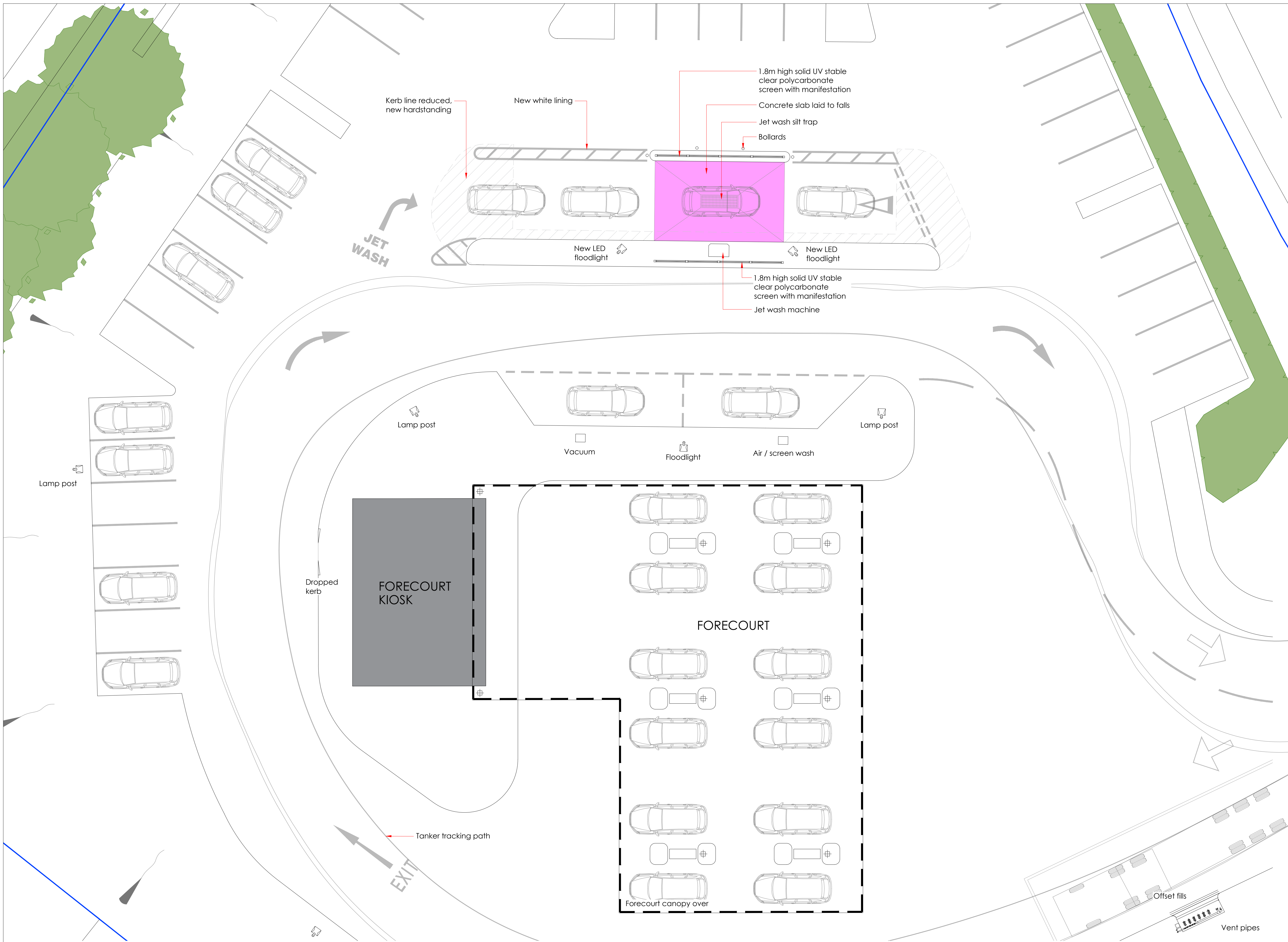
PROPOSED SITE LAYOUT
