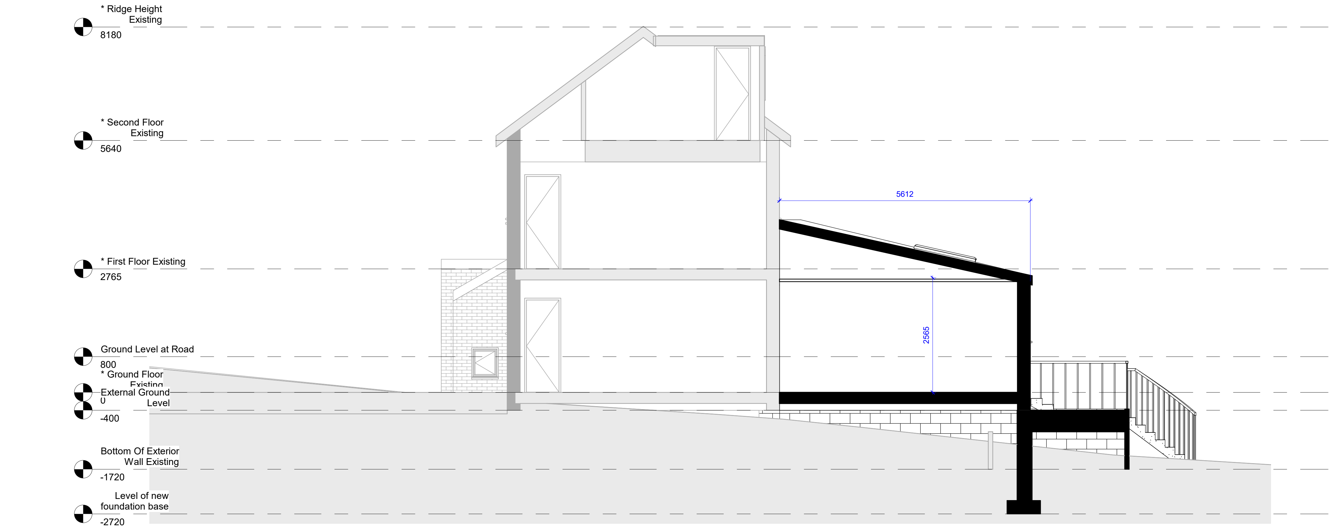
Section Through Showing Sloping Levels
