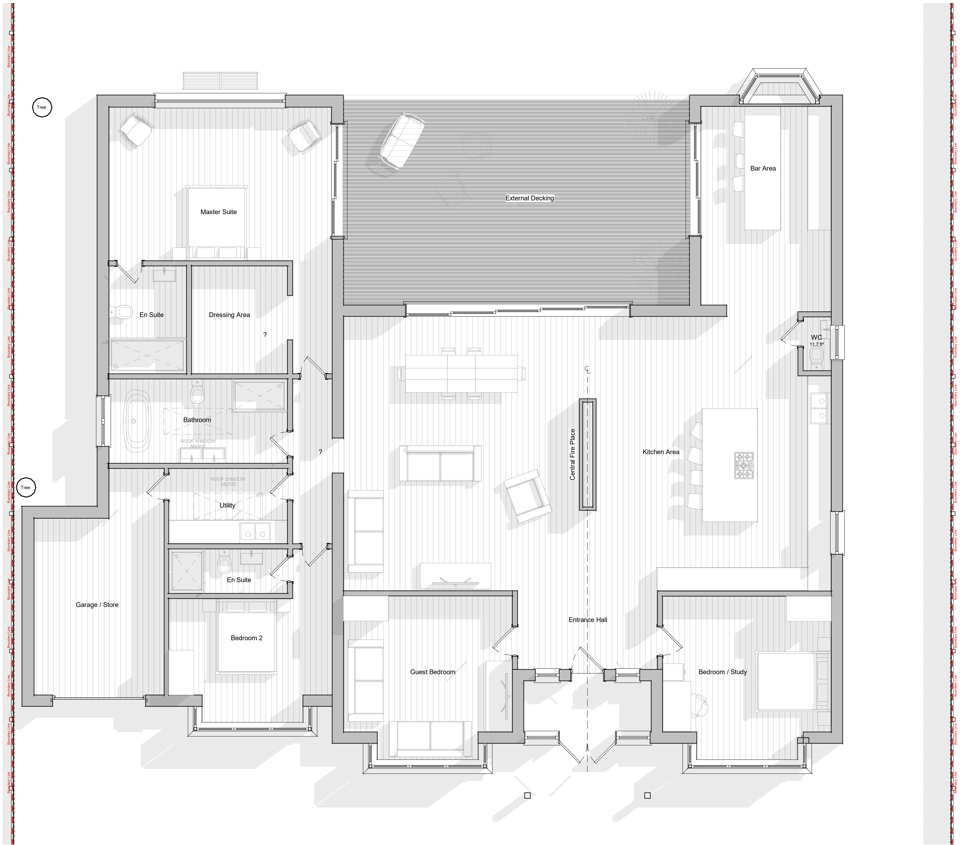
Proposed Ground Floor General Arrangement Layout 1 : 50
