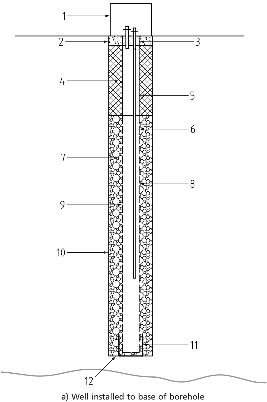
Figure 7 Typical well design
