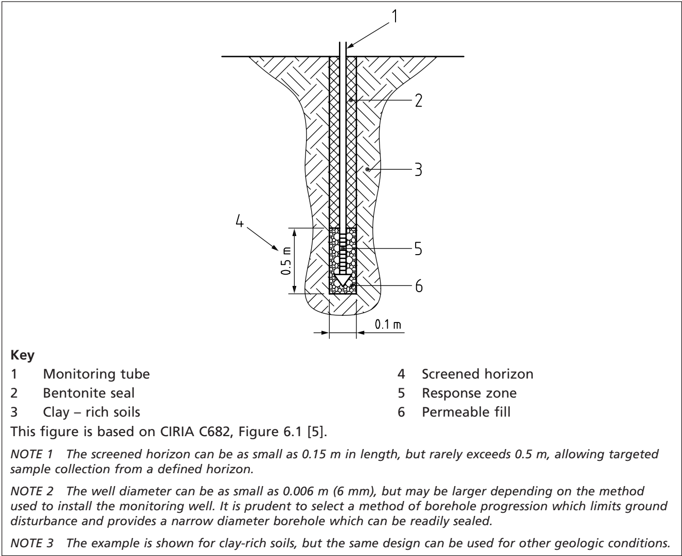
Figure 10 Example monitoring well construction for collection of ground gas samples for VOCs analysis
