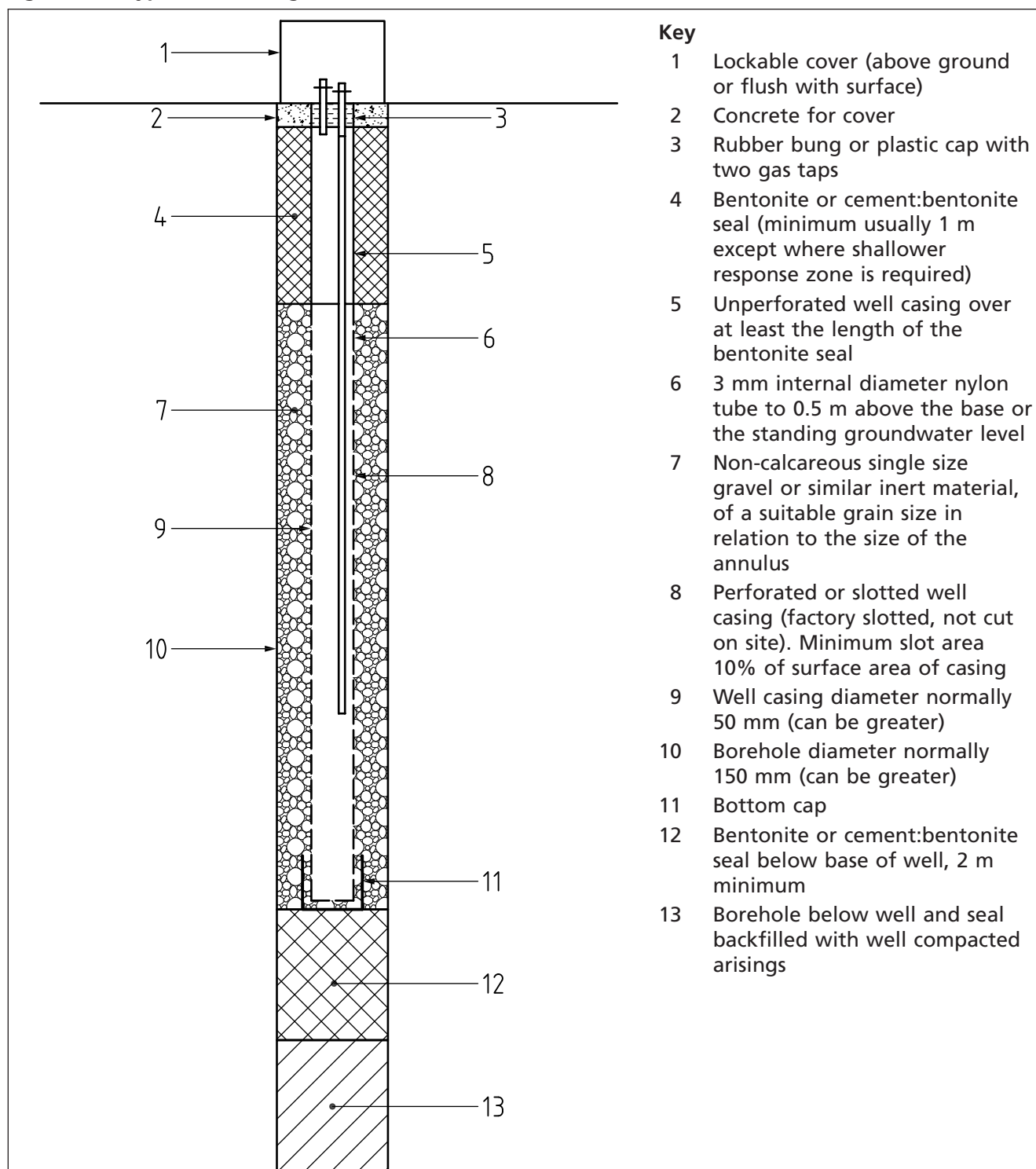
b) Well installed partway into borehole
