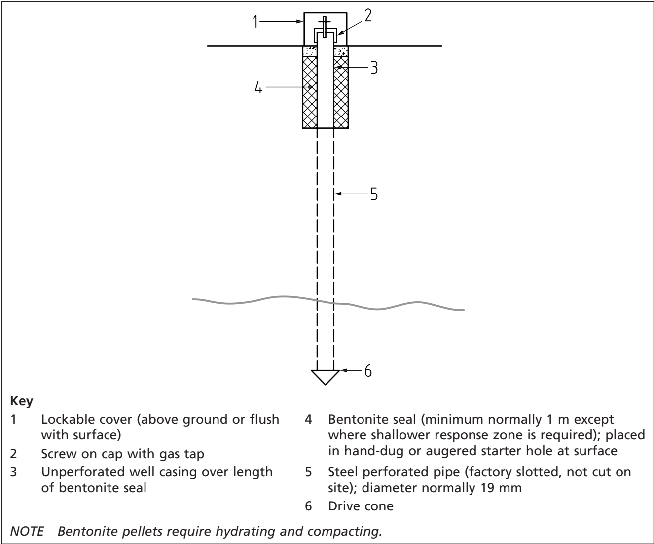
Figure 8 Driven monitoring probe
