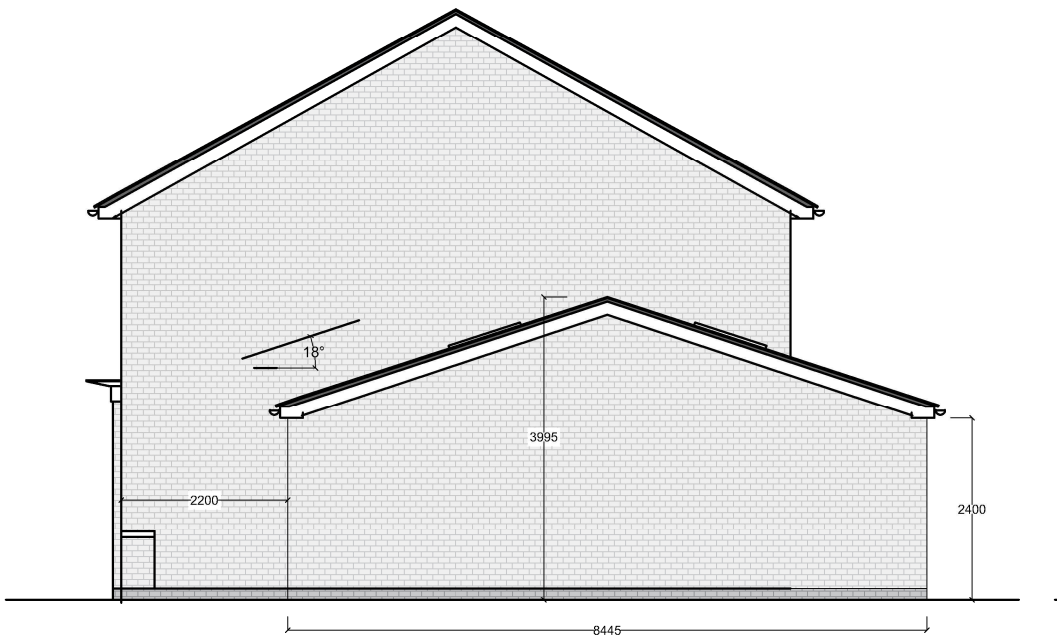
PROPOSED SIDE ELEVATION (Scale 1:100) SCALE BAR - (mm) 500 1000 2000
