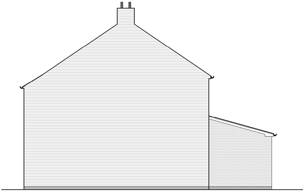
EXISTING SIDE ELEVATION (Scale 1:100) SCALE BAR - (mm) 500 1000 2000
