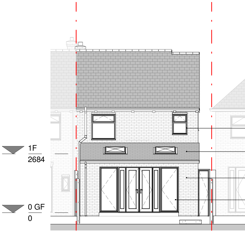
REAR ELEVATION
