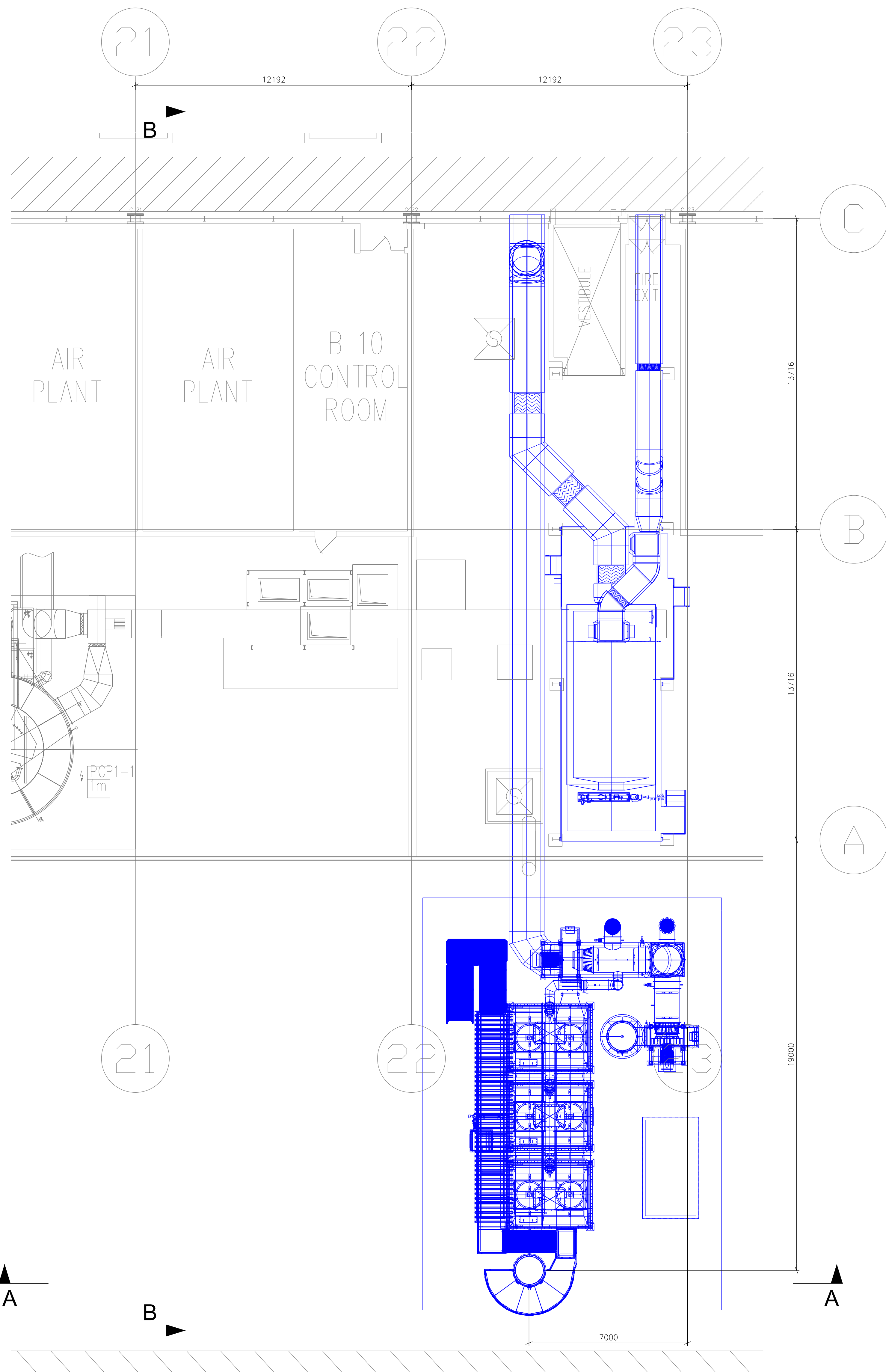
PROPOSED PLAN (+8m LVL.) Scale 1:100 @ A0
