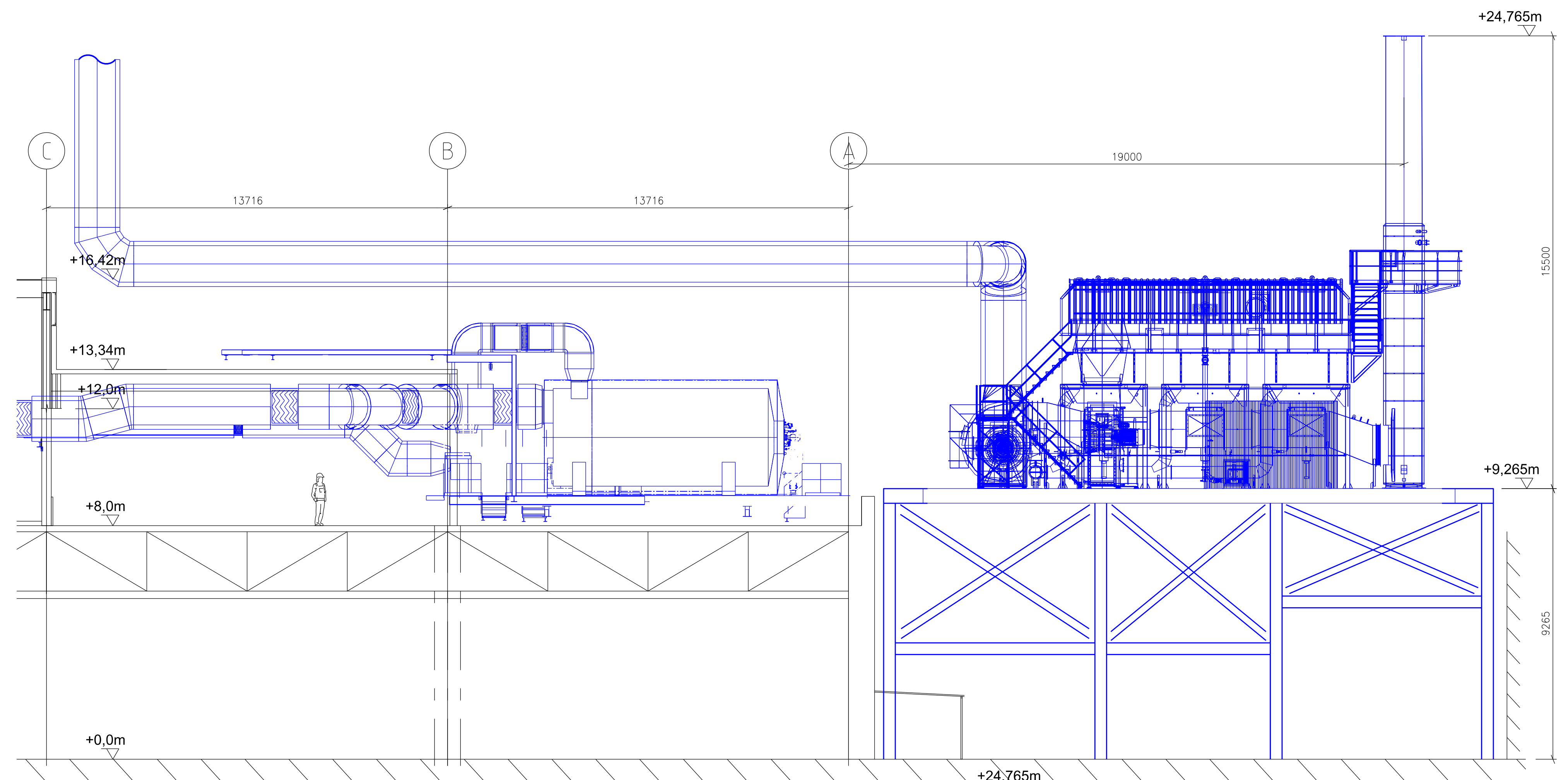
ELEVATION ACROSS SECTION B-B Scale 1:100 @ A0
