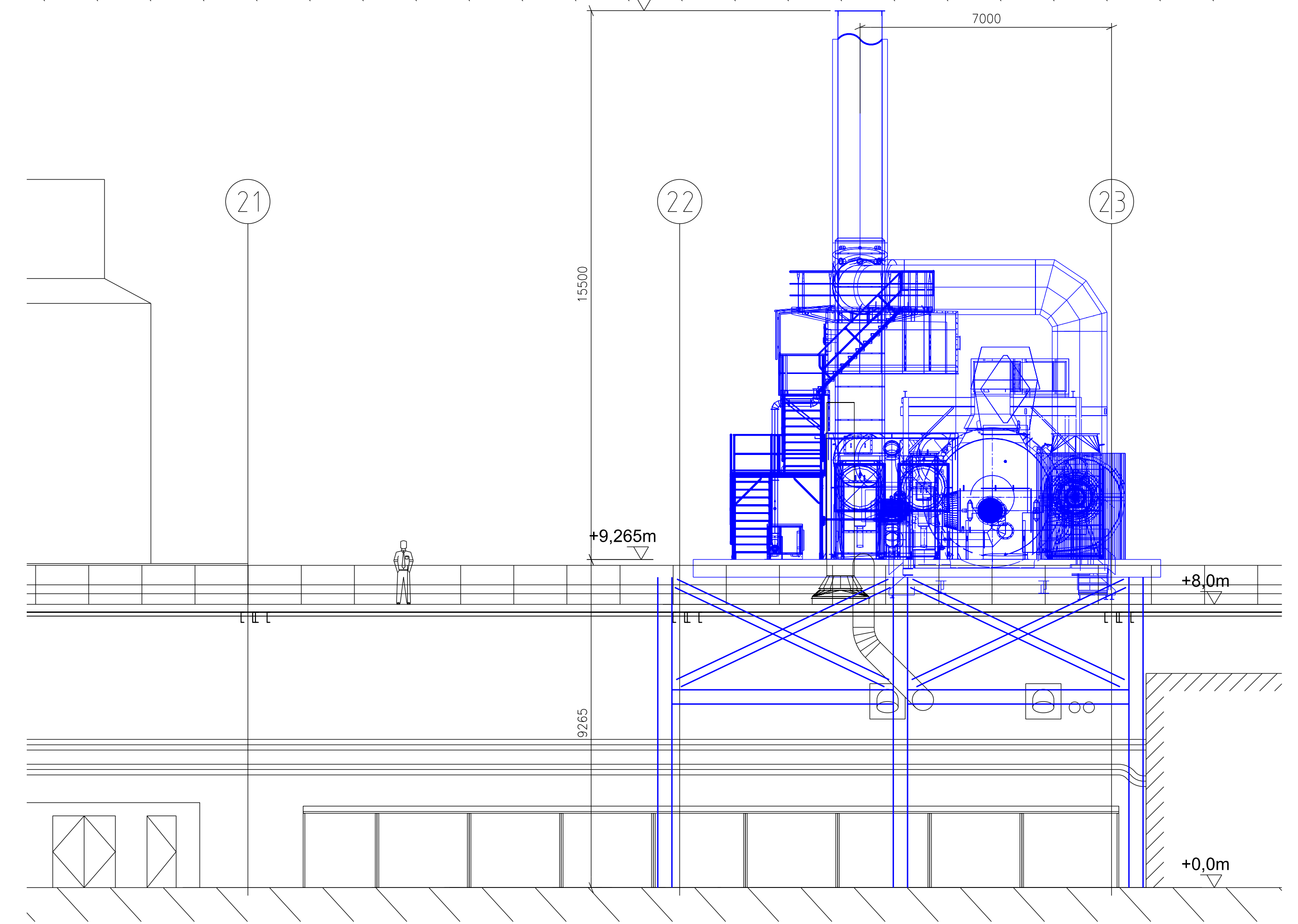
ELEVATION ACROSS SECTION A-A Scale 1:100 @ A0
