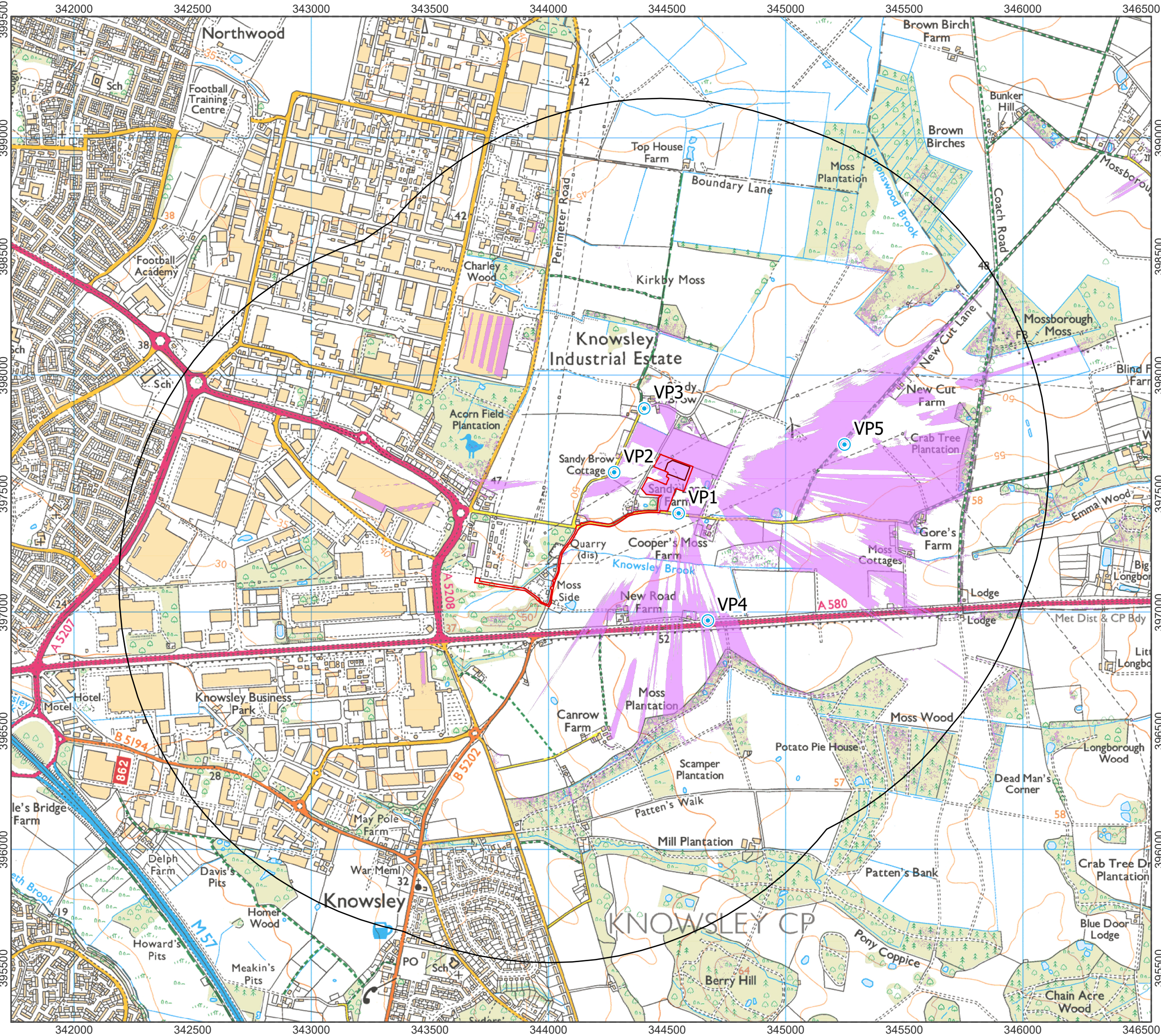
Figure 4 - Screened ZTV
