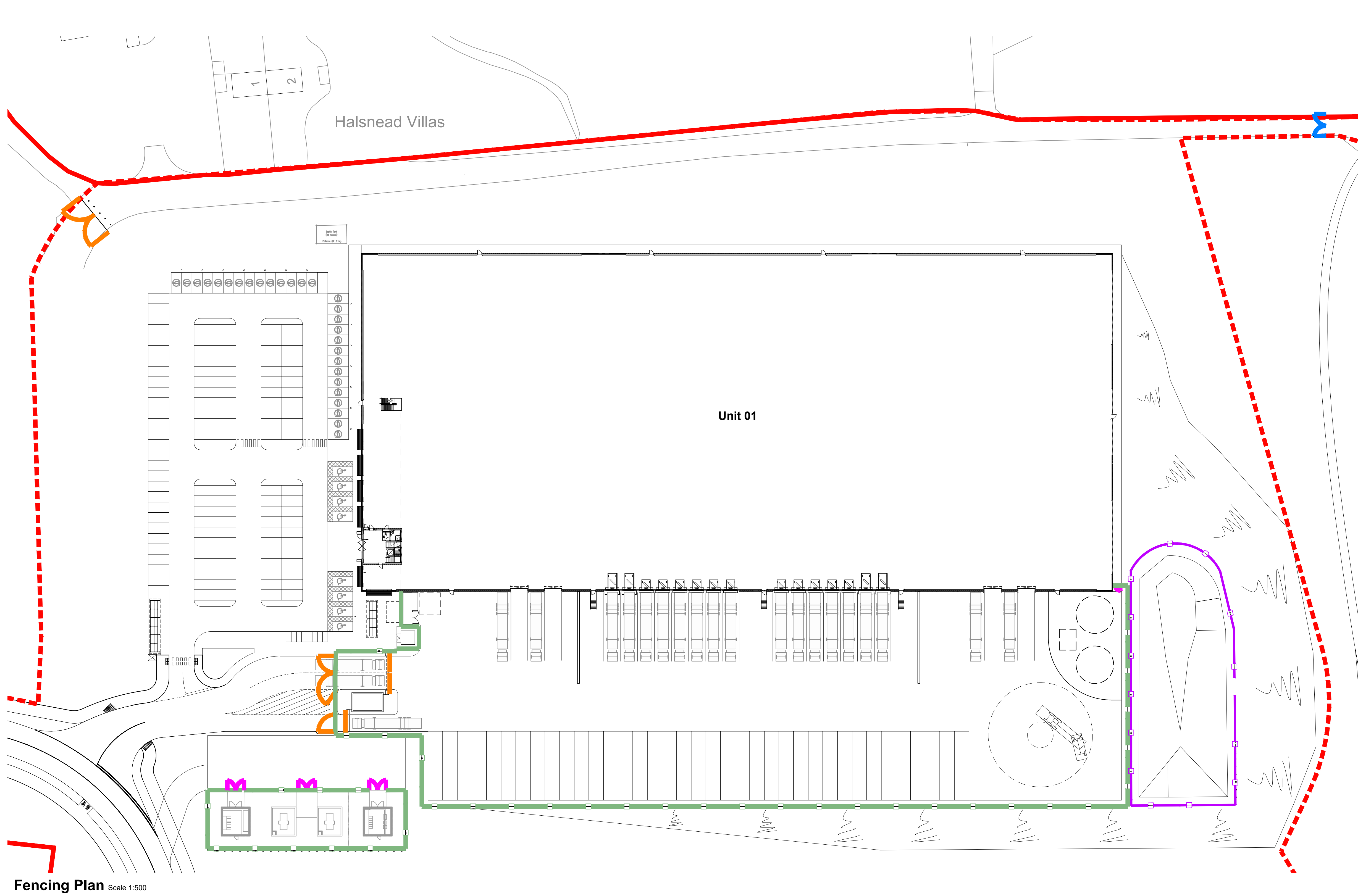
Fencing Plan Scale 1:500
