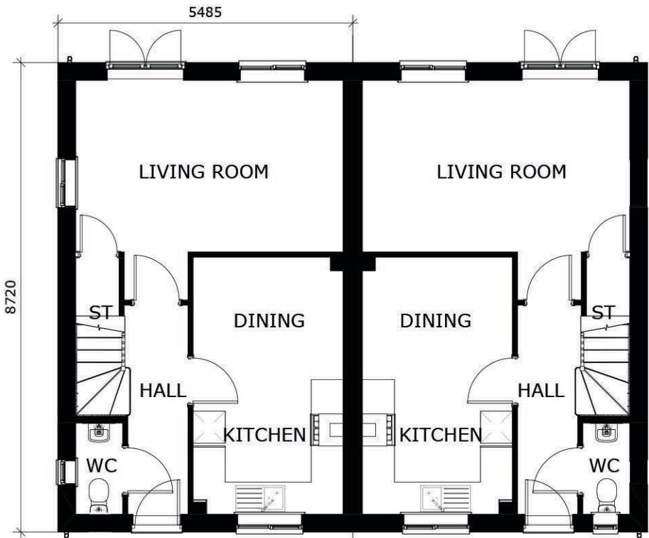
Plot 21 Plot 22 Ground Floor
