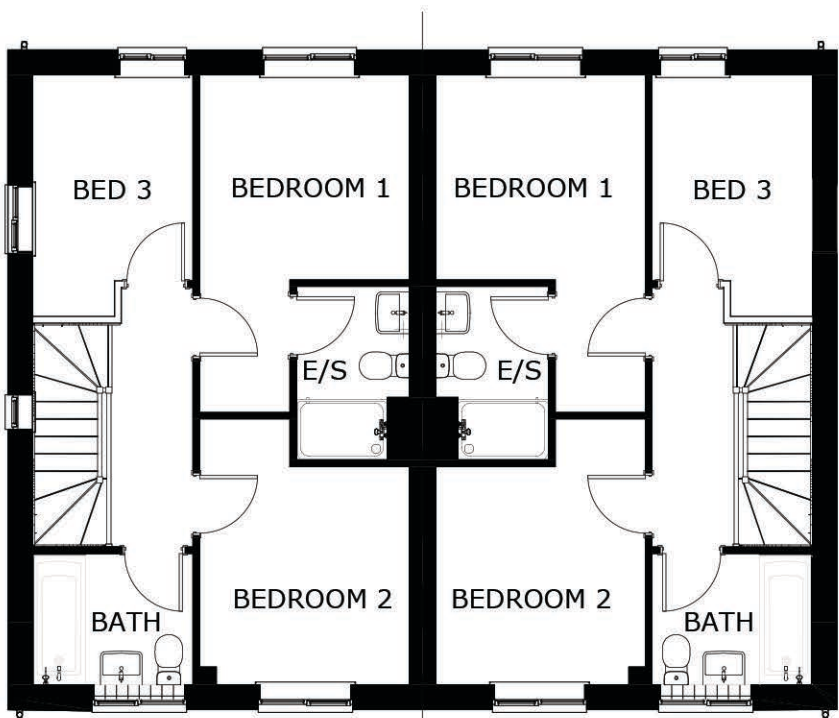
Plot 21 Plot 22 First Floor
