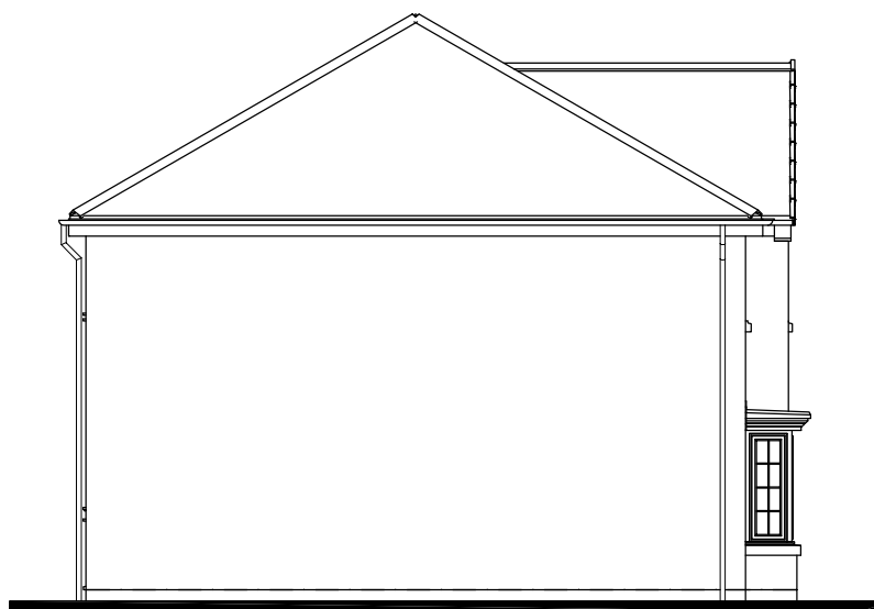
L.H. SIDE ELEVATION.
