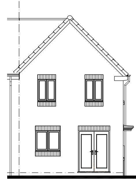
L.H. SIDE ELEVATION.
