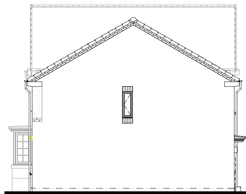
OVERTON SIDE ELEVATION.
