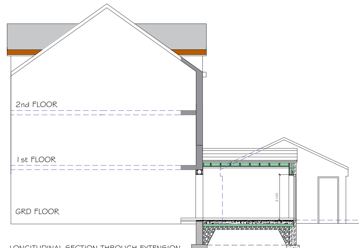
LONGITUDINAL SECTION THROUGH EXTENSION
