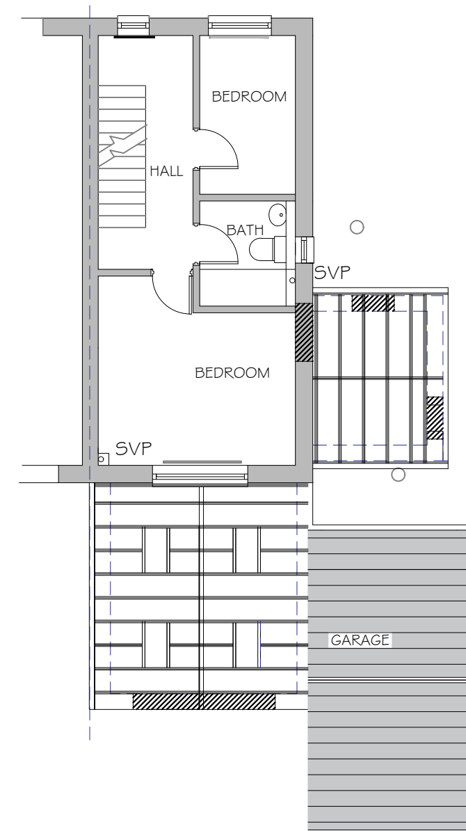
PROPOSED ROOF STRUCTURE AT FIRST FLOOR LEVEL
