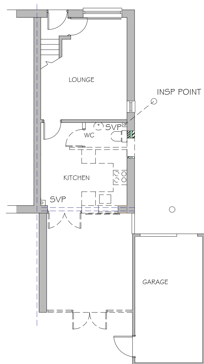
EXISTING GROUND FLOOR PLAN STRUCTURAL ALTERATIONS
