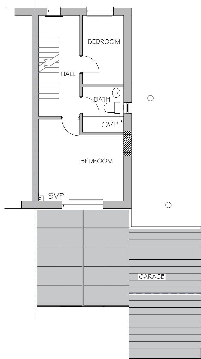
EXISTING FIRST FLOOR PLAN / ROOF PLAN
