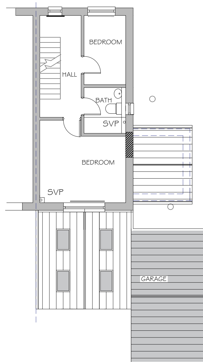
PROPOSED ROOF PLAN AT FIRST FLOOR LEVEL
