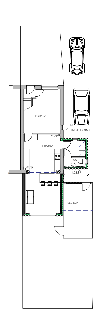
PROPOSED SITE PLAN 1:200
