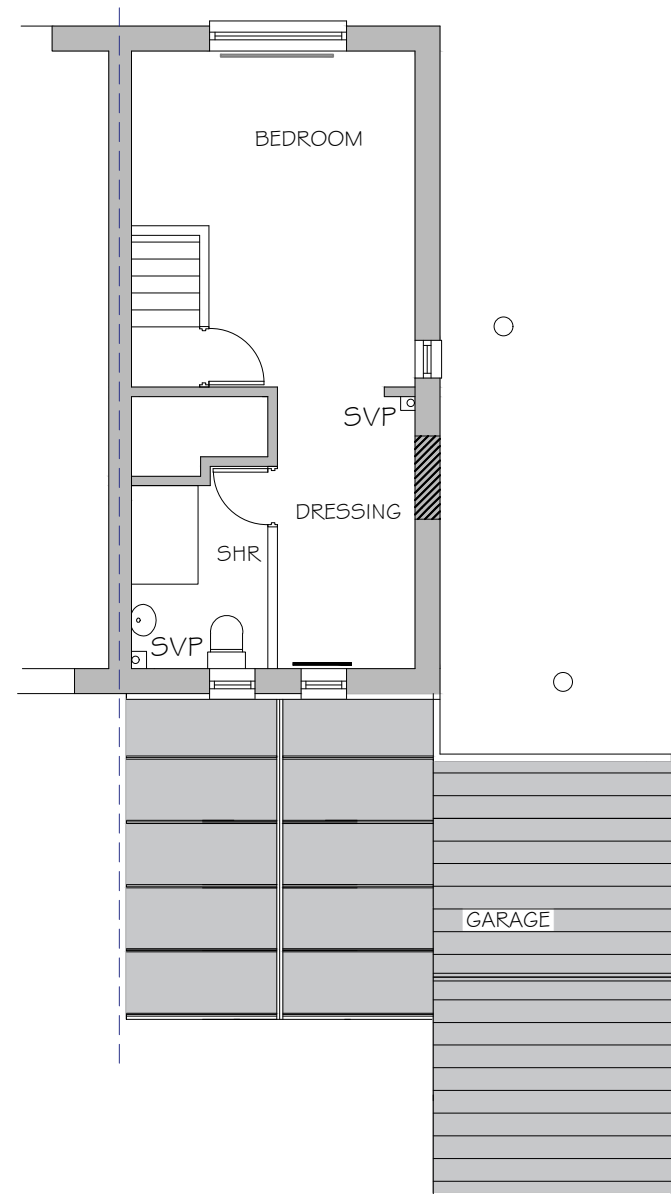
EXISTING SECOND FLOOR PLAN/ ROOF PLAN
