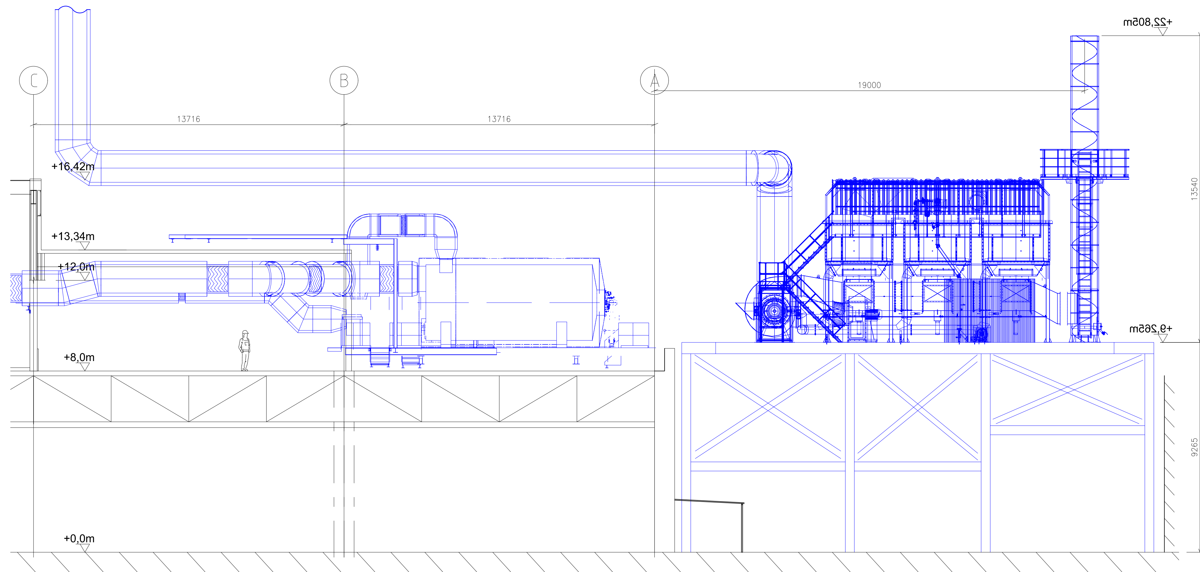
ELEVATION ACROSS SECTION B-B Scale 1:100 @ A0
