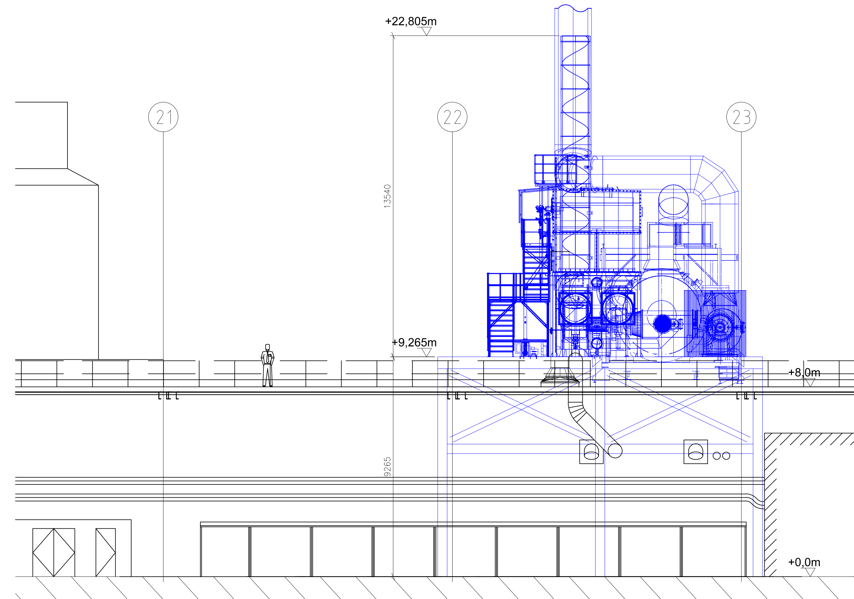
ELEVATION ACROSS SECTION A-A Scale 1:100 @ A0
