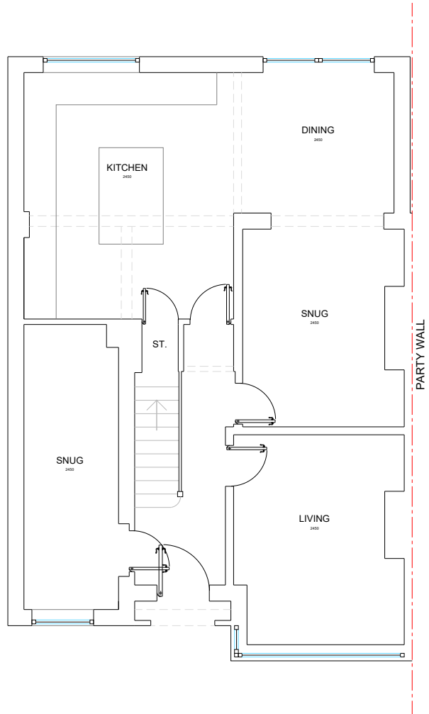
GROUND FLOOR
