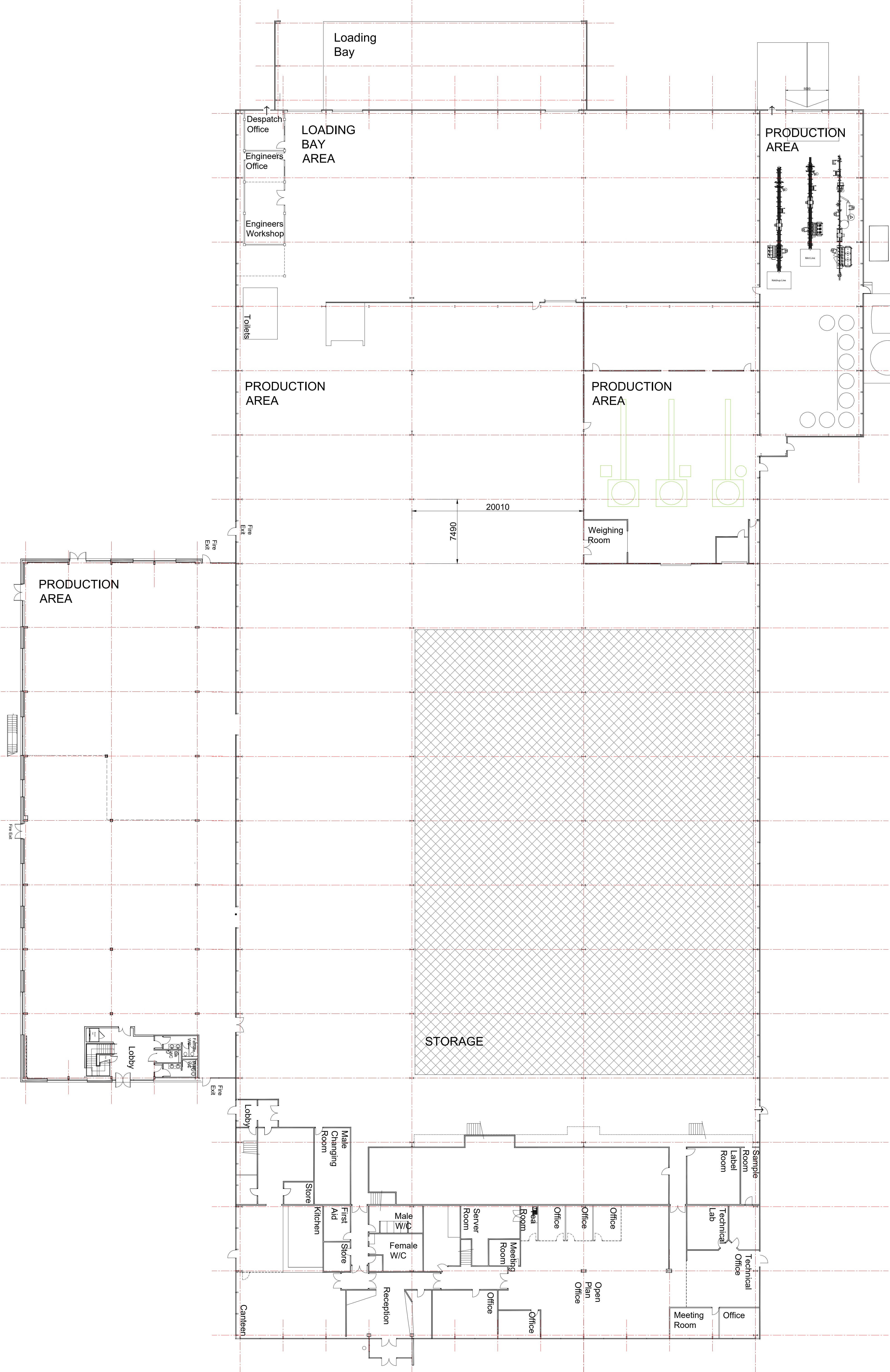
Ground Floor Plan as existing @ 1:200
