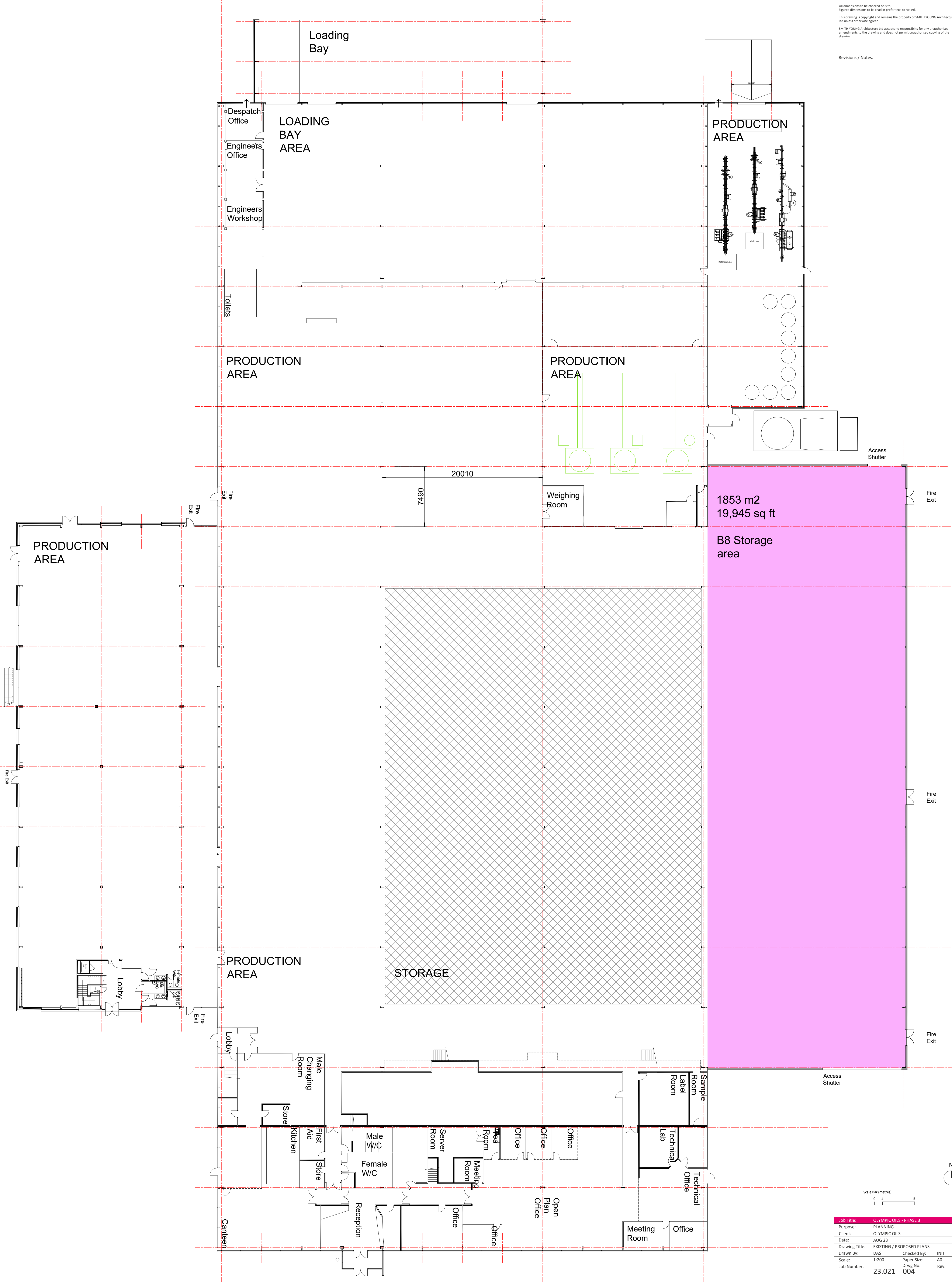
Ground Floor Plan as PROPOSED @ 1:200
