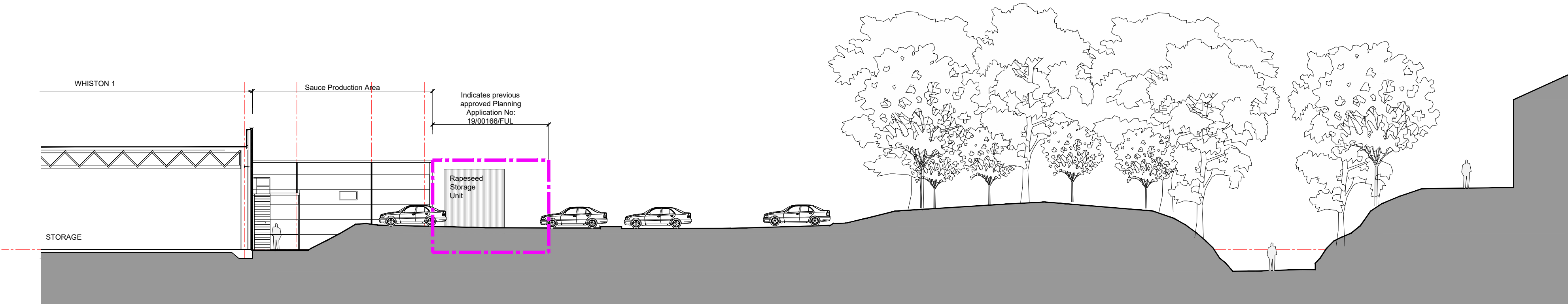
Section B-B as Existing @ 1:200
