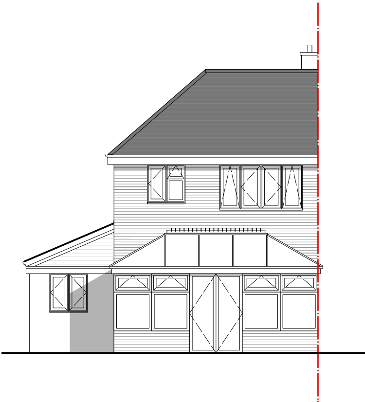
PROPOSED WEST ELEVATION
