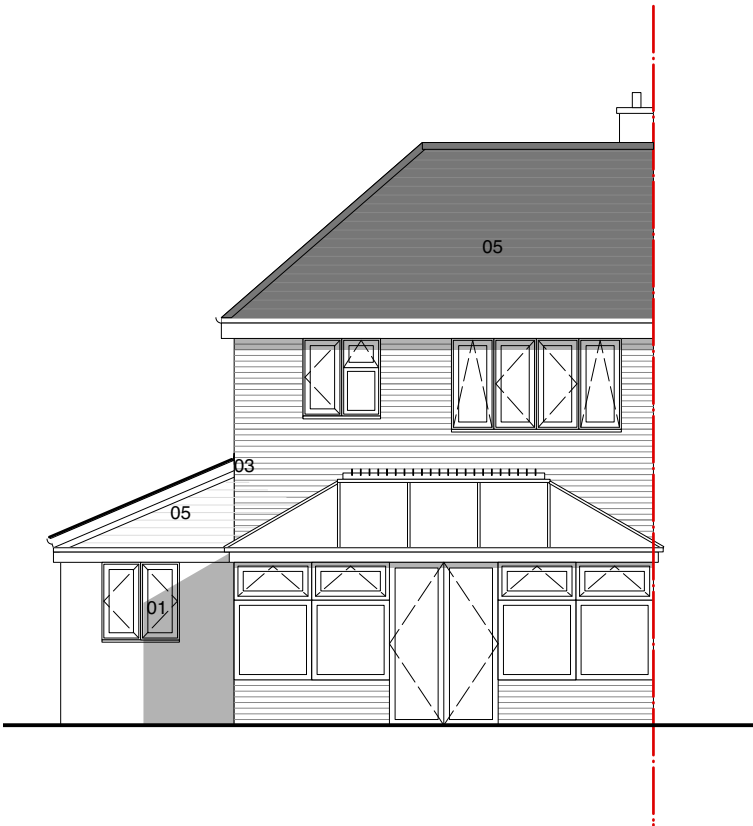
EXISTING WEST ELEVATION
