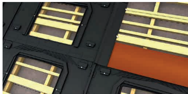
Installation of lateral flashing
