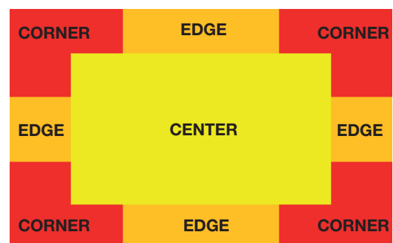
One-sloped roof
