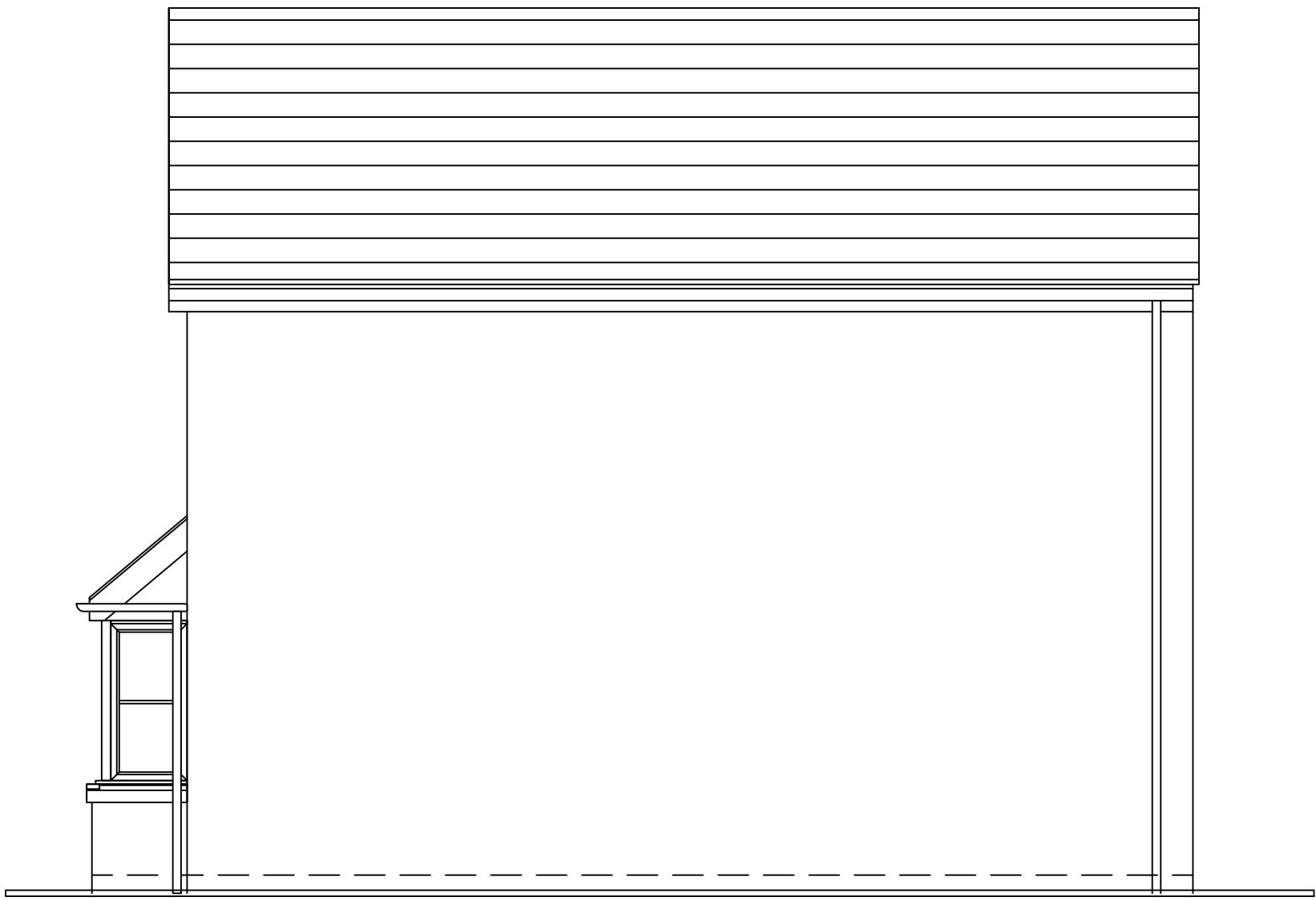
SIDE ELEVATION
