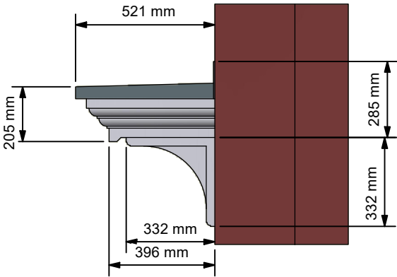
Side Elevation ( 1 : 20 )
