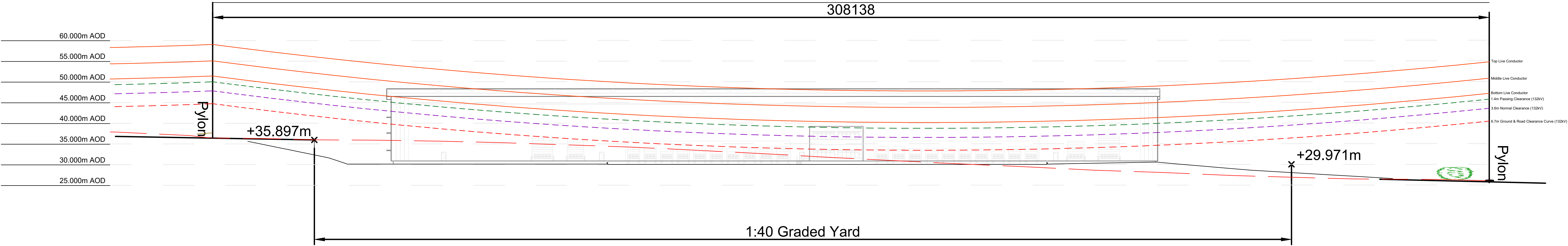
Site Section Below Cable Path Scale 1:500
