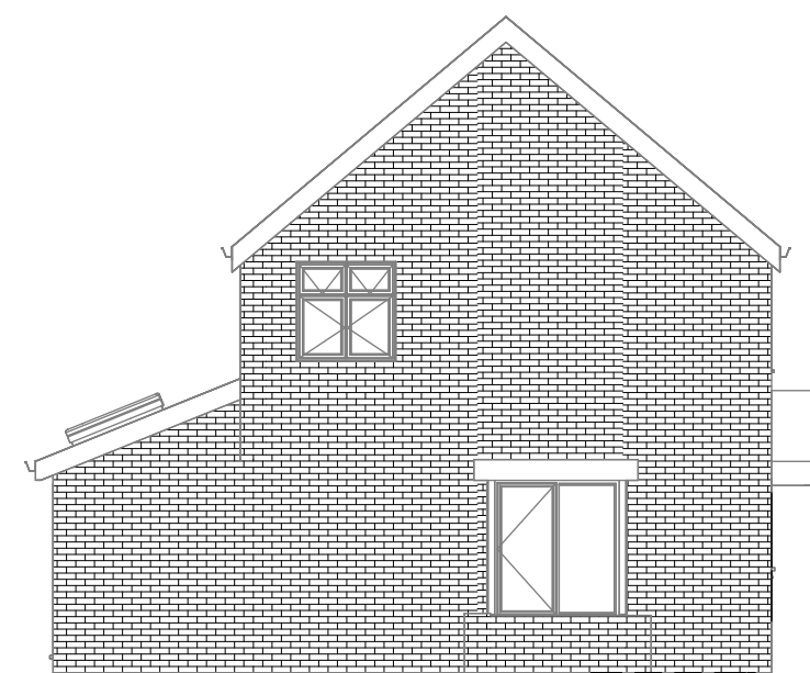
14 Proposed Side Extension 2 1 : 100
