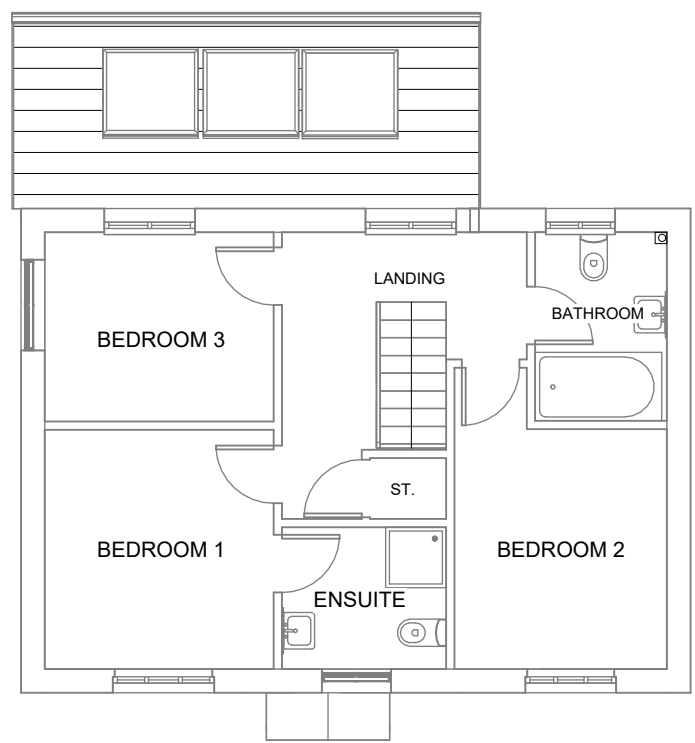
9 Proposed 1F 1 : 100
