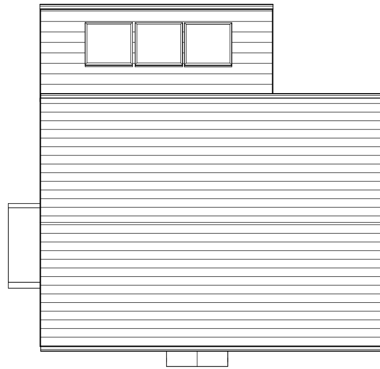
3 Existing Roof Plan 1 : 100
