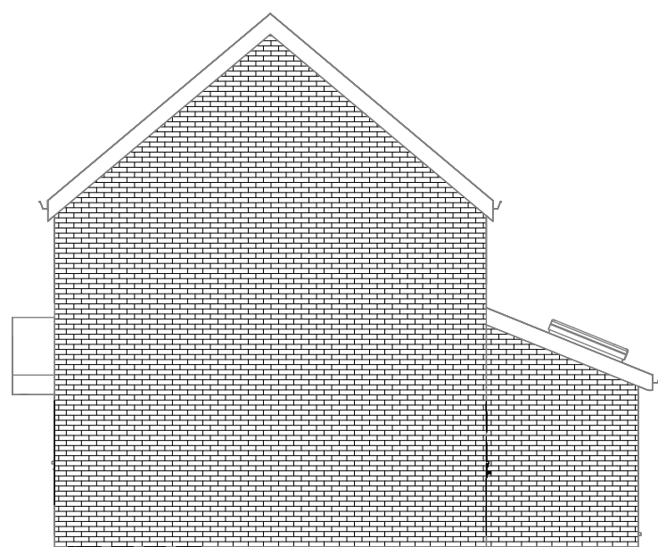
13 Proposed Side Elevation 1 : 100
