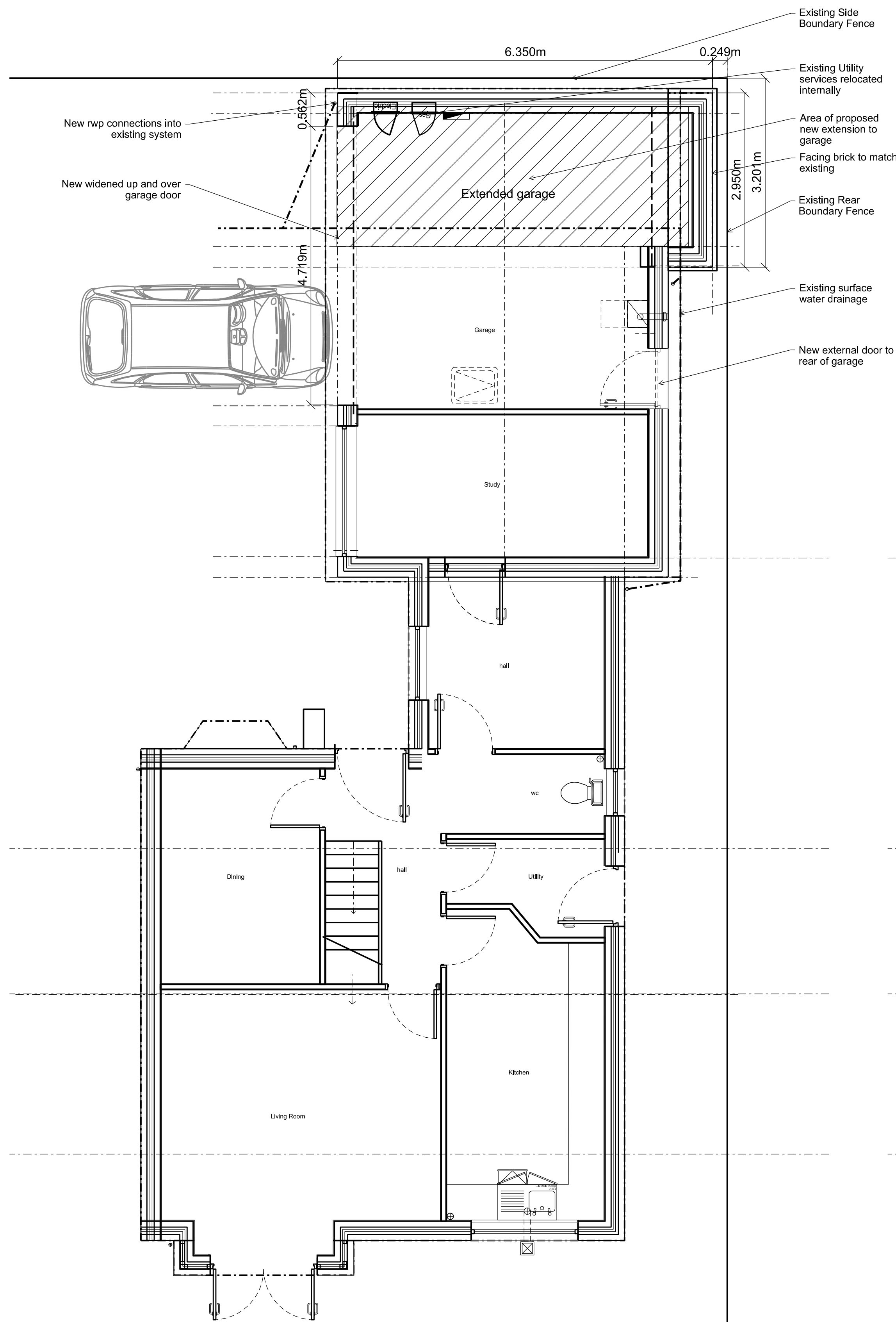
Proposed Ground Floor
