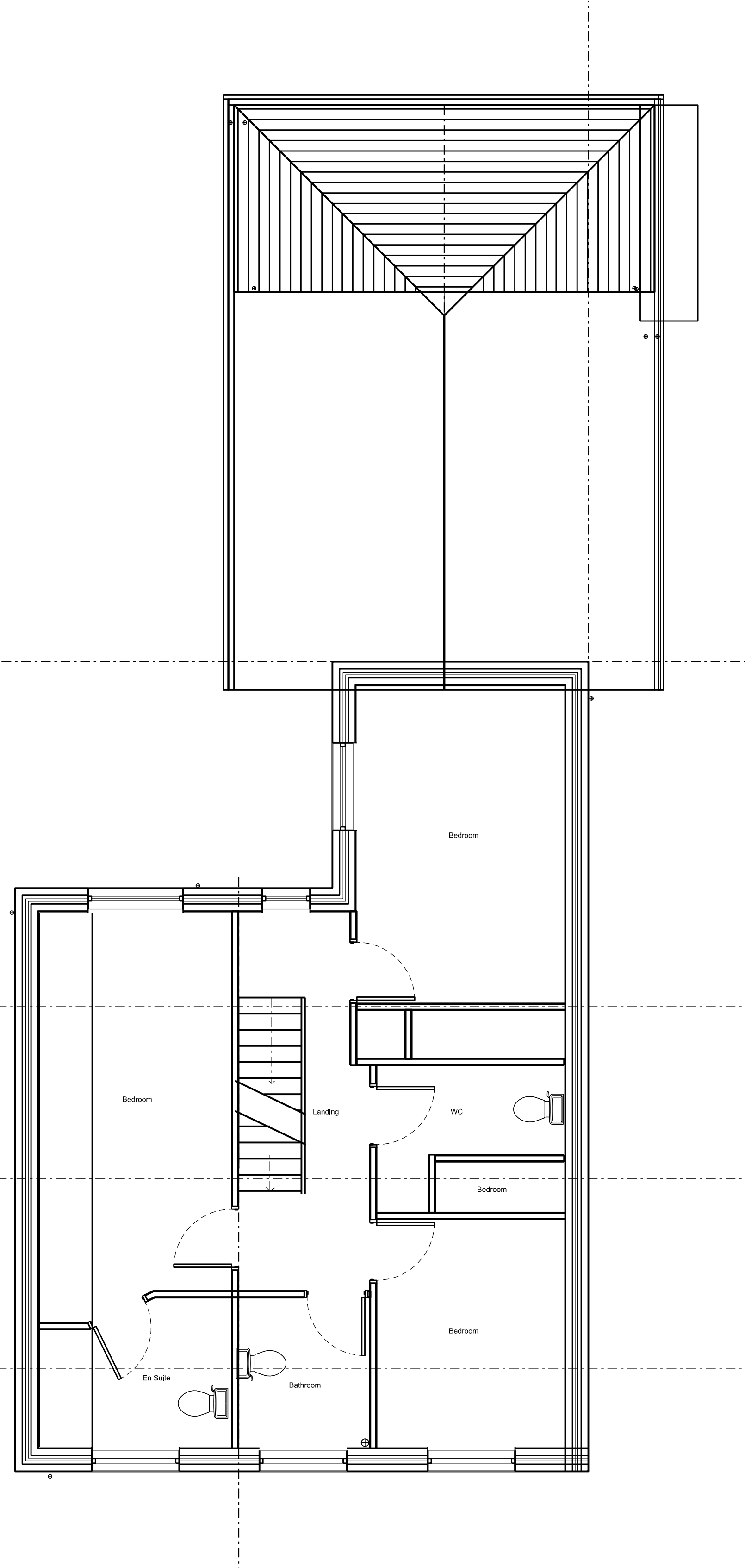
Proposed First Floor
