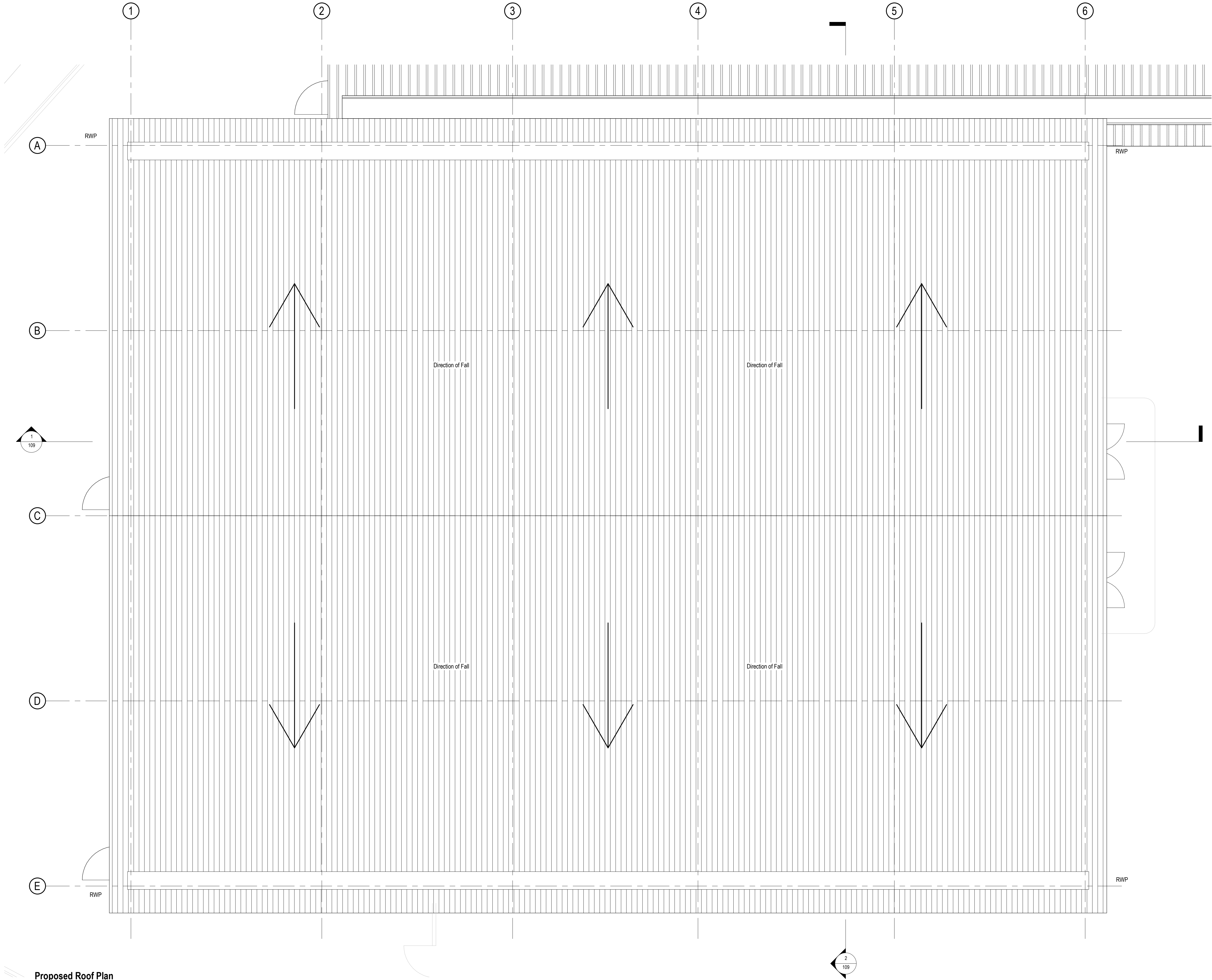
Proposed Roof Plan 1 : 50
