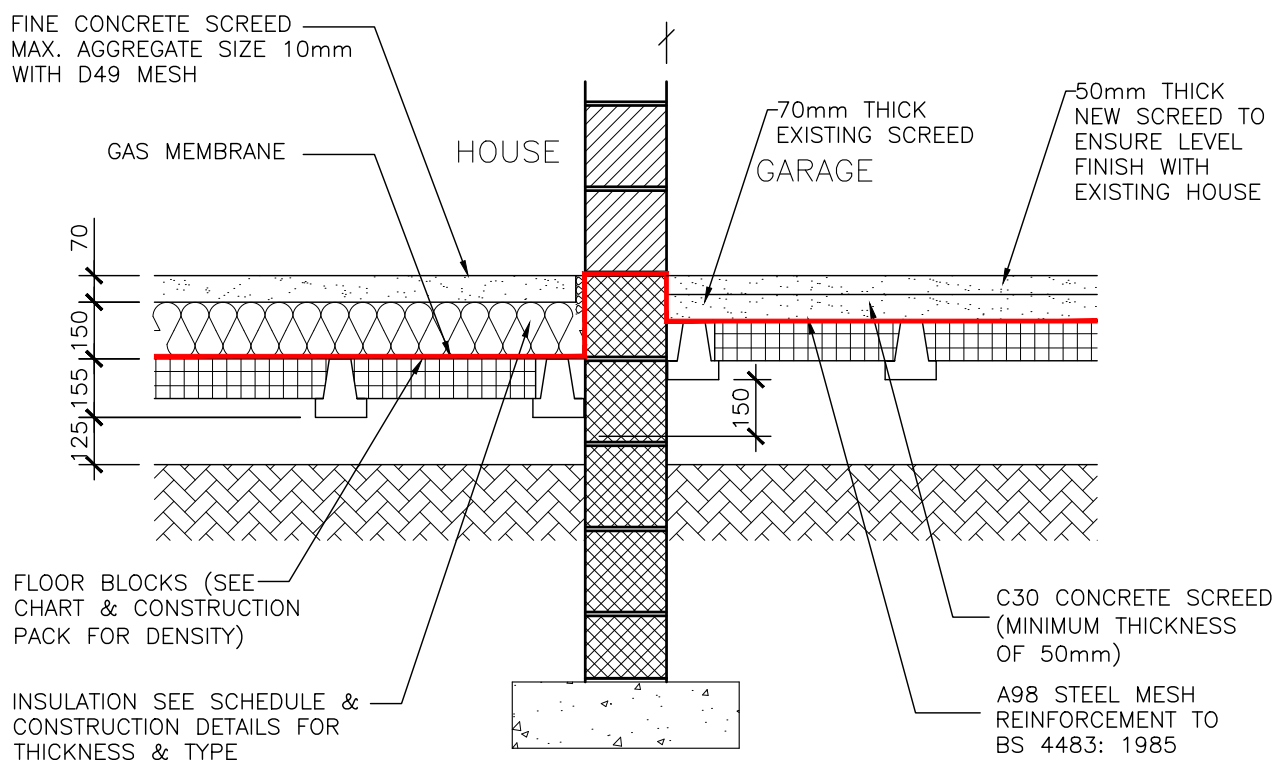
LEVEL GARAGE/ HOUSE SLAB DETAILS
