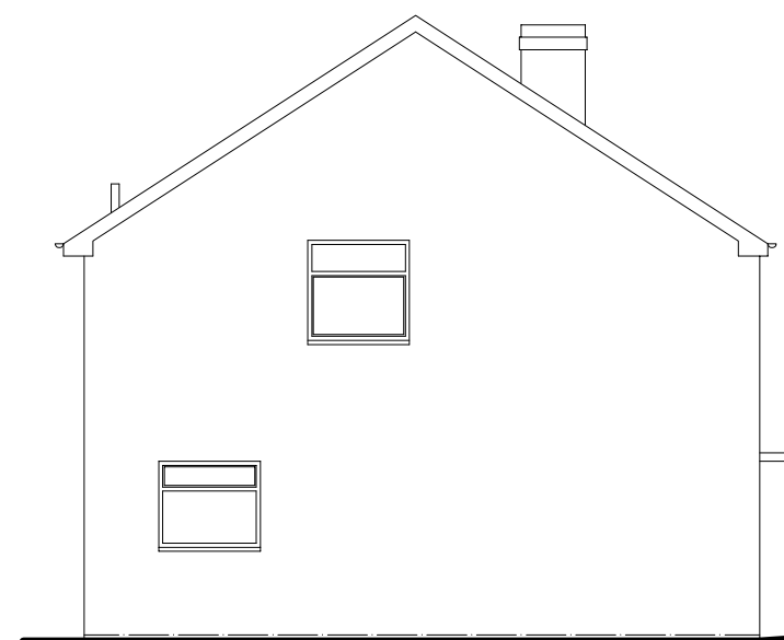
Existing side (south) elevation @ 1:100 scale
