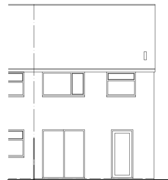
Existing rear elevation @ 1:100 scale
