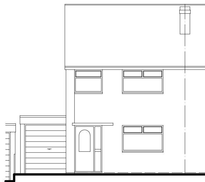
Existing front elevation @ 1:100 scale
