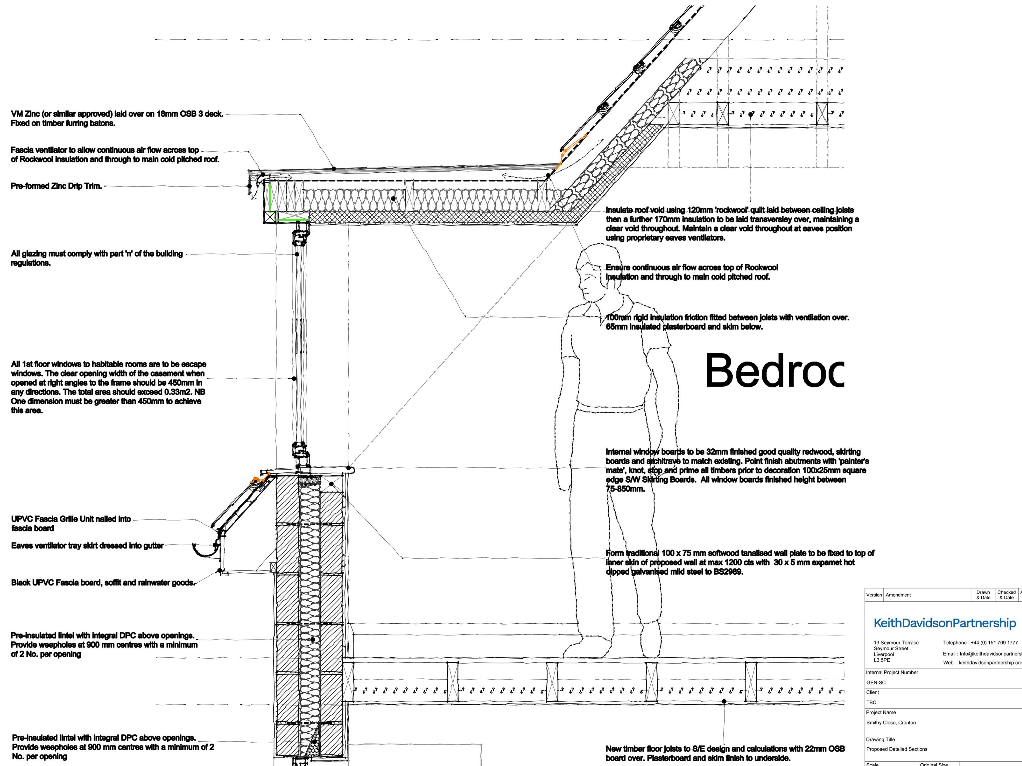
TYPICAL SECTION DETAIL 2 (Scale 1:10)
