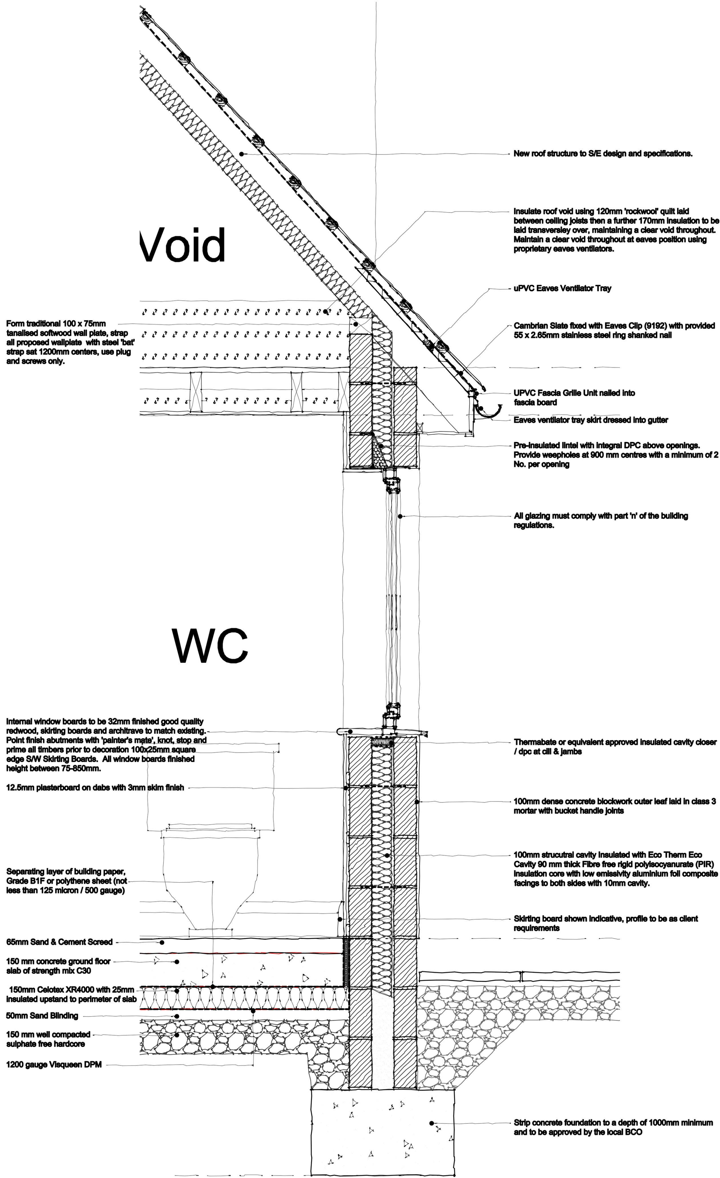
TYPICAL SECTION DETAIL 1 (Scale 1:10)
