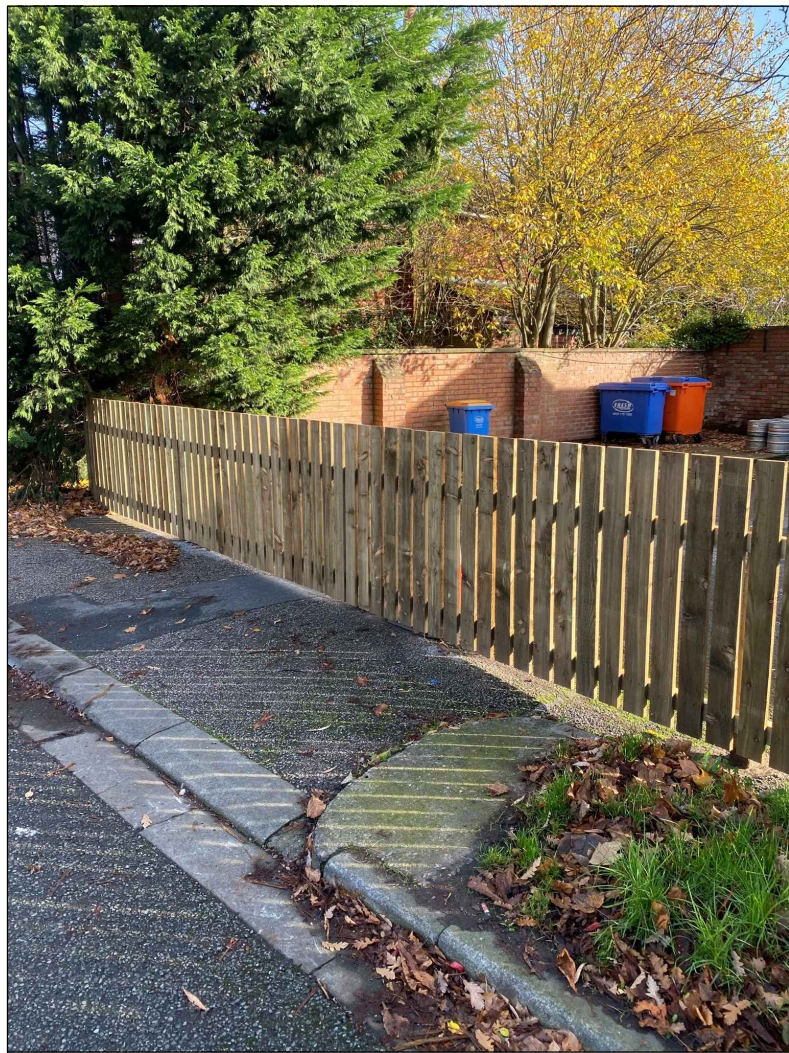
DESIGN INTENT EXTERNAL GARDEN FENCE DETAIL 02 IMG 01
