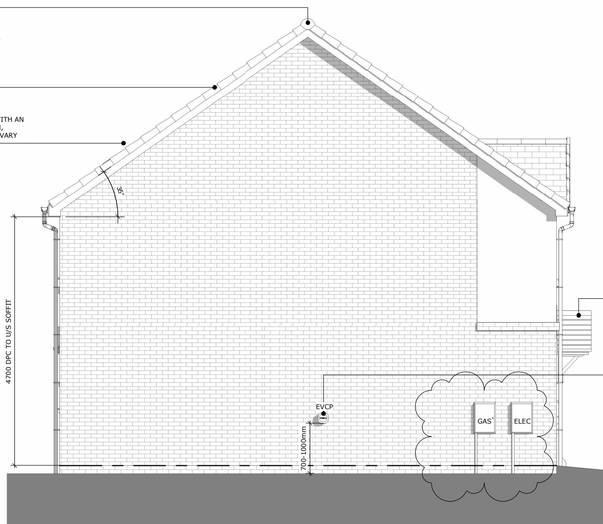
LEFT HAND SIDE ELEVATION
