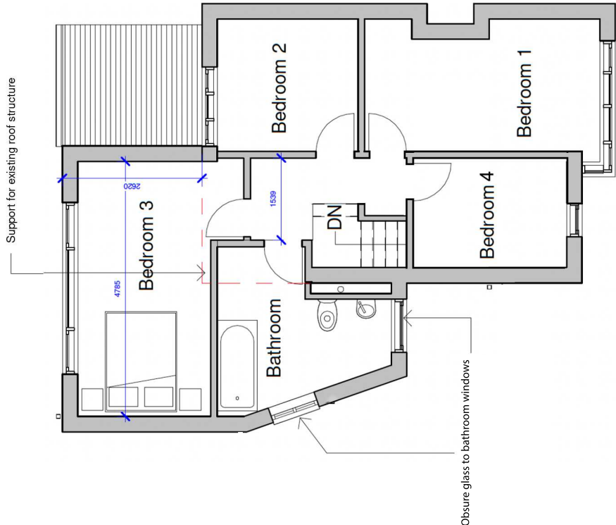
First Floor 1 : 100
