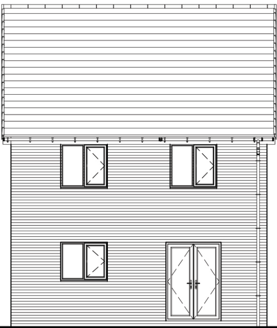
Rear Elevation
