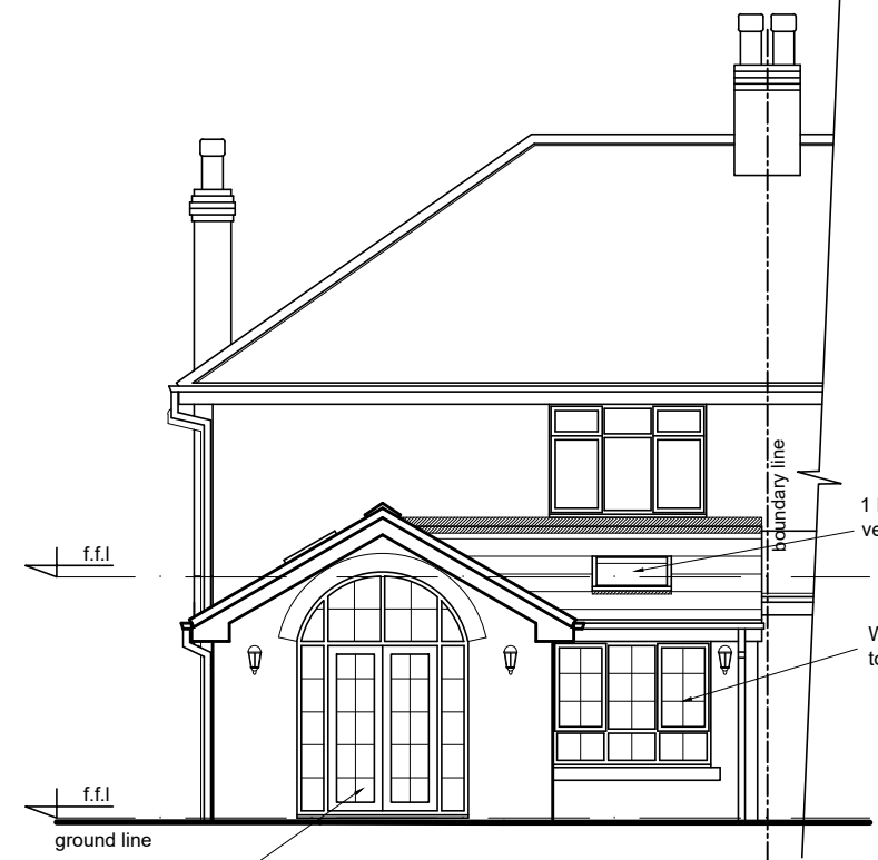
REAR ELEVATION
