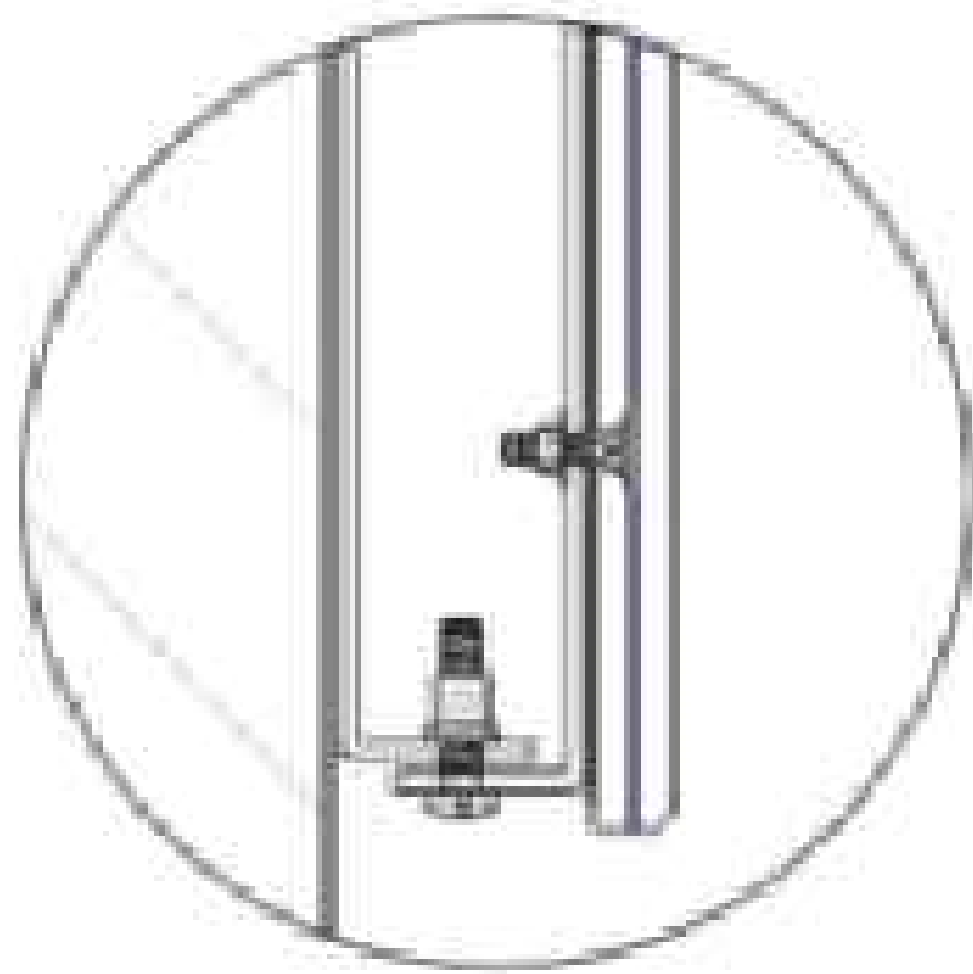
Surround Detail 1:1
