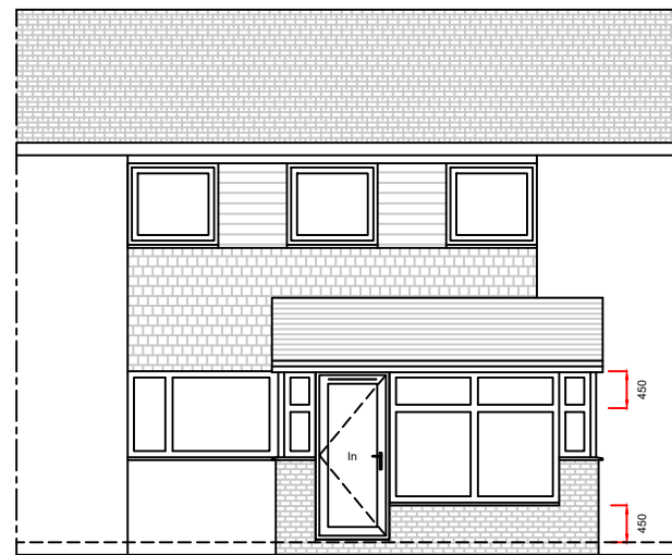
Front Elevation
