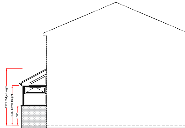
Right-Hand Side Elevation
