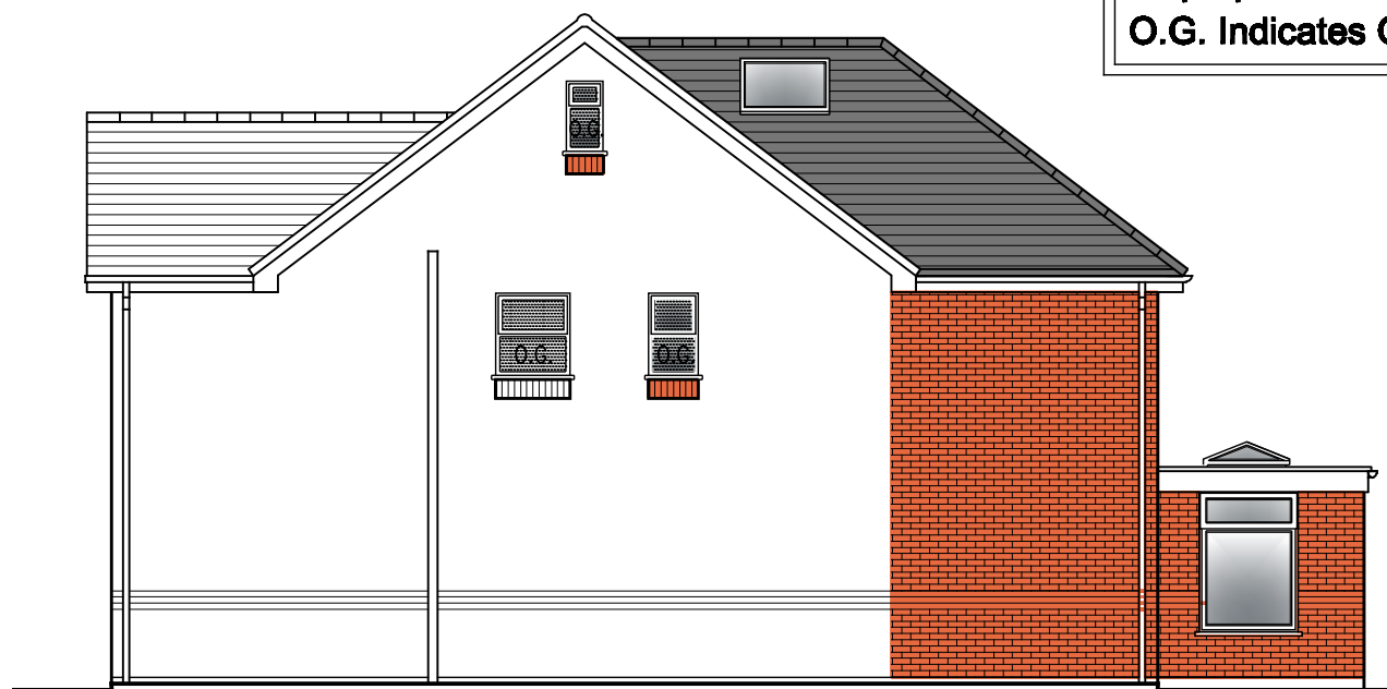
Proposed Side Elevation. West Facing
