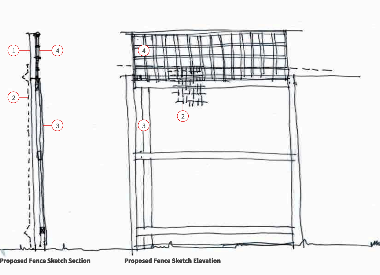
Proposed Fence B-C
