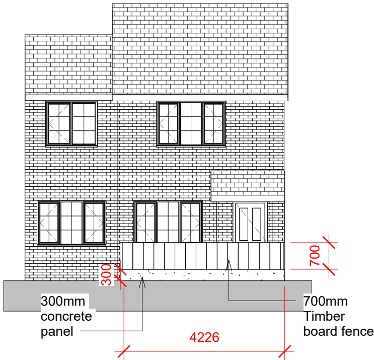
Front Elevation 1 : 100
