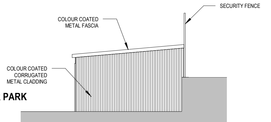
ELEVATION C
