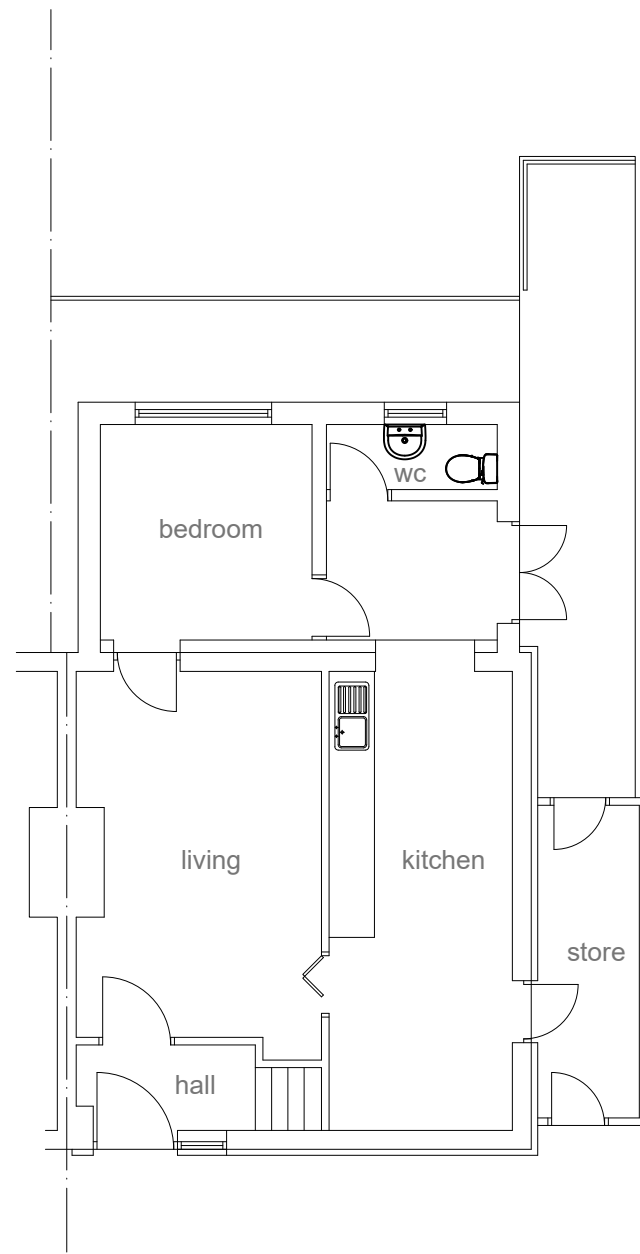
Existing ground floor plan @ 1:100 scale
