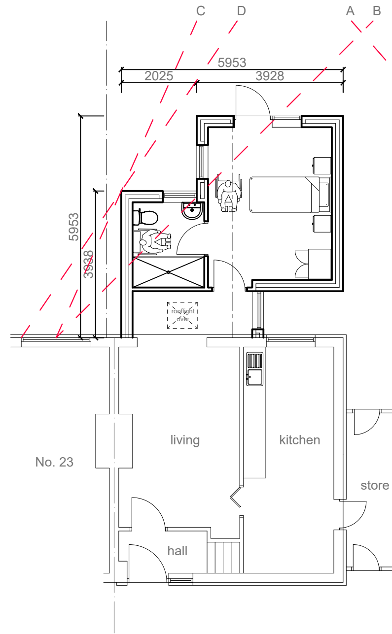
Proposed ground floor plan @ 1:100 scale DRAFT 2
