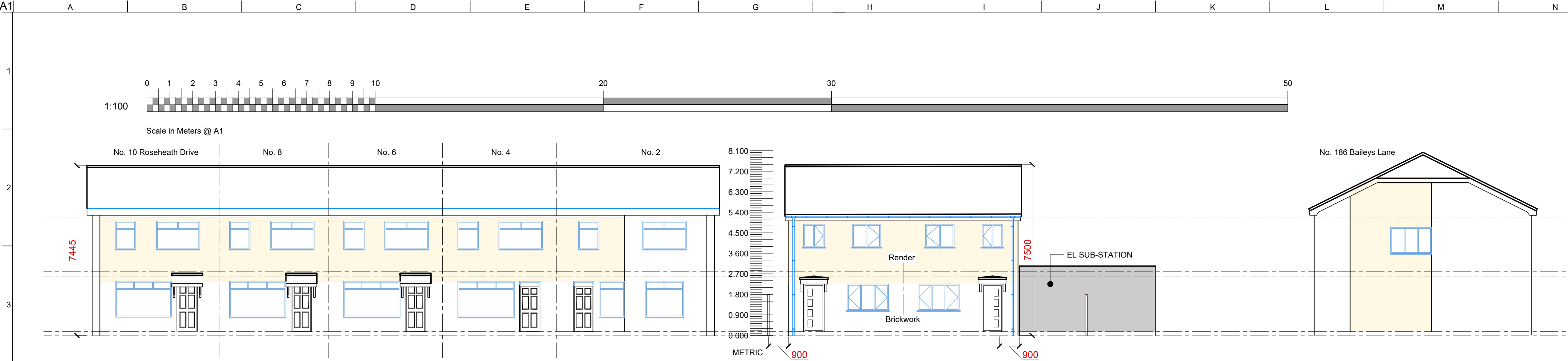
ROAD ROSEHEATH DRIVE - BAILEYS LANE STREET SCENE Scale: 1:100 @ A1
